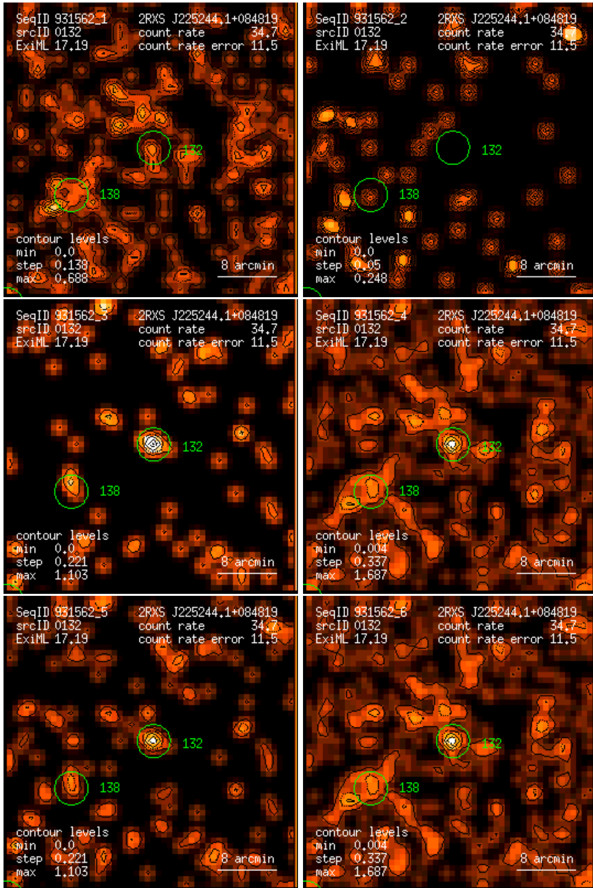
Figure 132: RASS 931562: detection 0132: band rate images, Gaussian filter: (1) PSPC channels 11 – 41, (2) 52 – 90, (3) 91 – 201, (4) 11 – 235, (5) 52 – 201, (6) 11 – 201. Broad band rates in counts/ks. Band rate contour levels in counts/ks/arcmin 2 .
