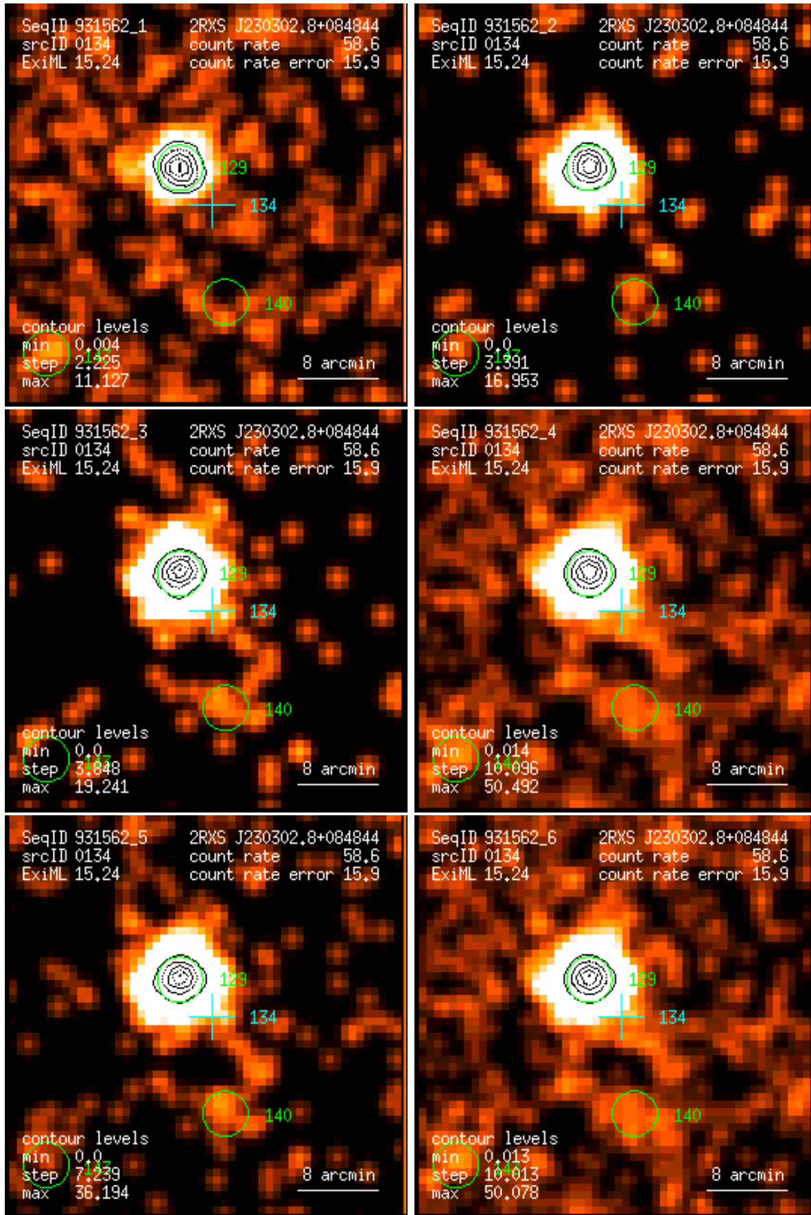
Figure 134: RASS 931562: detection 0134: band rate images, Gaussian filter: (1) PSPC channels 11 – 41, (2) 52 – 90, (3) 91 – 201, (4) 11 – 235, (5) 52 – 201, (6) 11 – 201. Broad band rates in counts/ks. Band rate contour levels in counts/ks/arcmin 2 .
