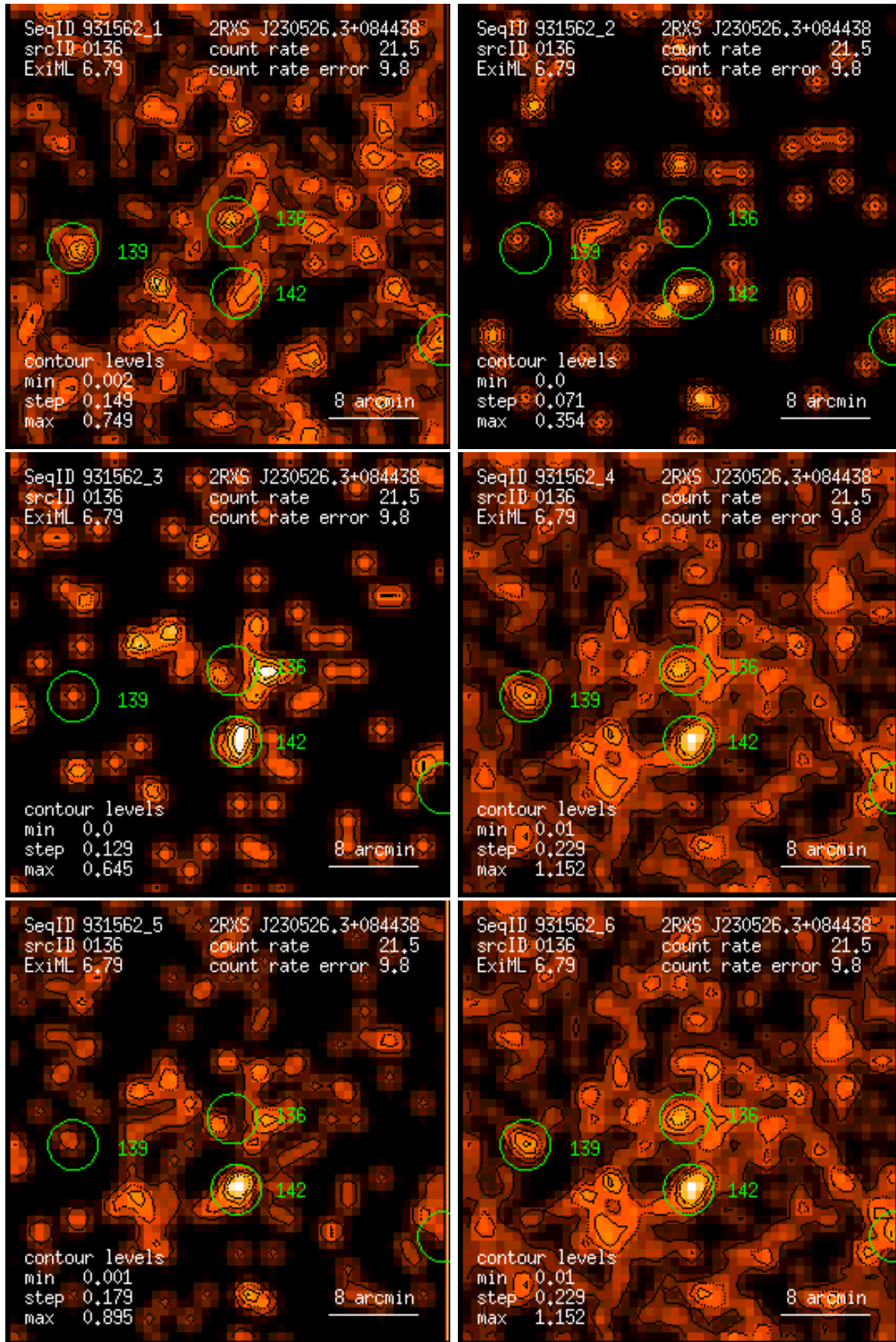
Figure 136: RASS 931562: detection 0136: band rate images, Gaussian filter: (1) PSPC channels 11 – 41, (2) 52 – 90, (3) 91 – 201, (4) 11 – 235, (5) 52 – 201, (6) 11 – 201. Broad band rates in counts/ks. Band rate contour levels in counts/ks/arcmin 2 .
