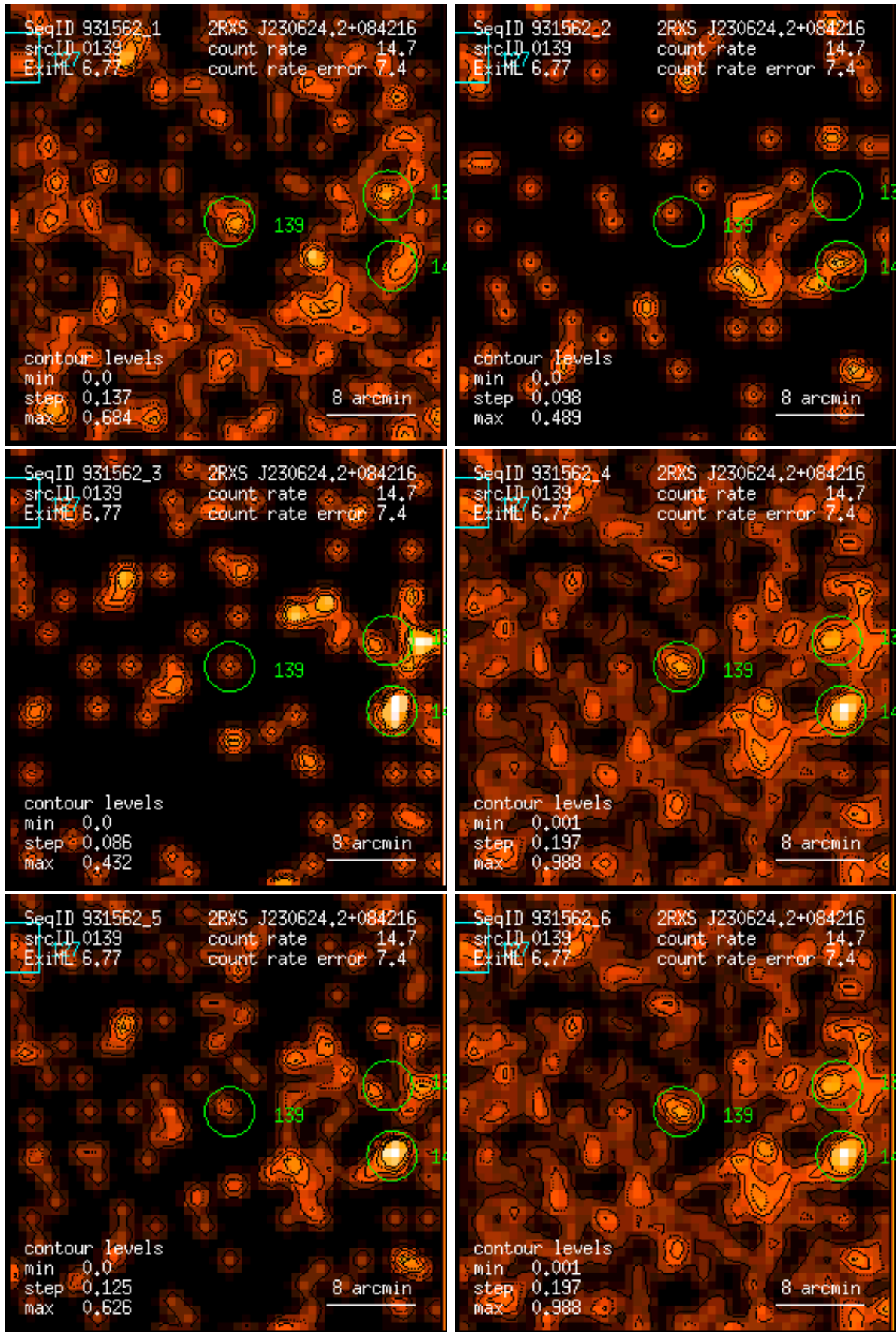
Figure 139: RASS 931562: detection 0139: band rate images, Gaussian filter: (1) PSPC channels 11 – 41, (2) 52 – 90, (3) 91 – 201, (4) 11 – 235, (5) 52 – 201, (6) 11 – 201. Broad band rates in counts/ks. Band rate contour levels in counts/ks/arcmin 2 .
