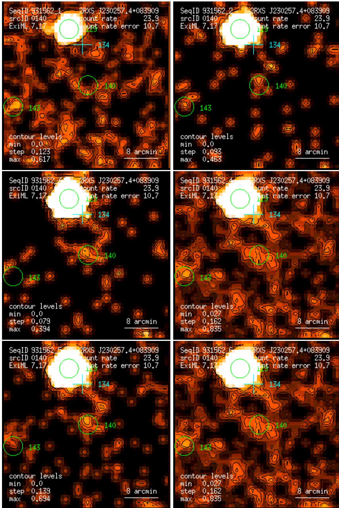
Figure 140: RASS 931562: detection 0140: band rate images, Gaussian filter: (1) PSPC channels 11 – 41, (2) 52 – 90, (3) 91 – 201, (4) 11 – 235, (5) 52 – 201, (6) 11 – 201. Broad band rates in counts/ks. Band rate contour levels in counts/ks/arcmin 2 .
