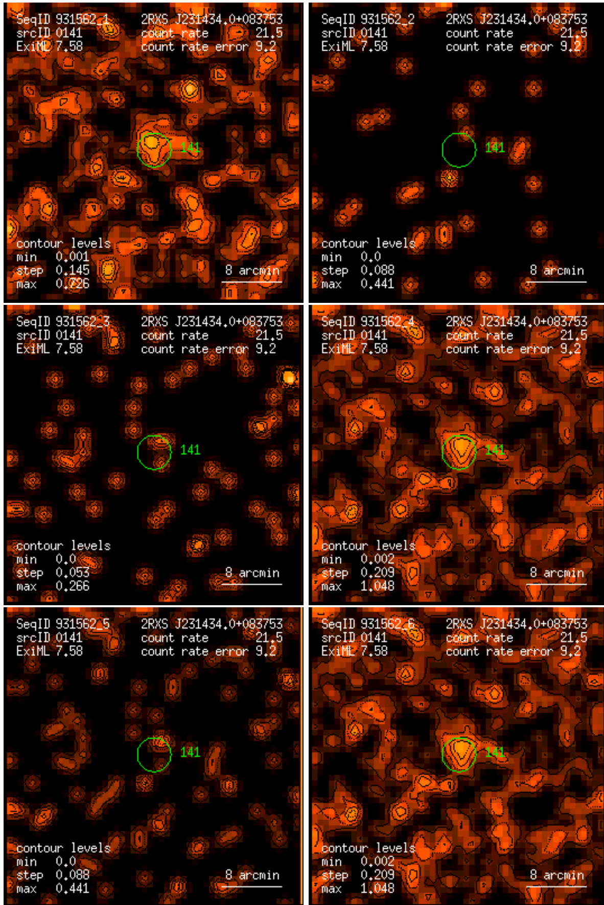
Figure 141: RASS 931562: detection 0141: band rate images, Gaussian filter: (1) PSPC channels 11 – 41, (2) 52 – 90, (3) 91 – 201, (4) 11 – 235, (5) 52 – 201, (6) 11 – 201. Broad band rates in counts/ks. Band rate contour levels in counts/ks/arcmin 2 .
