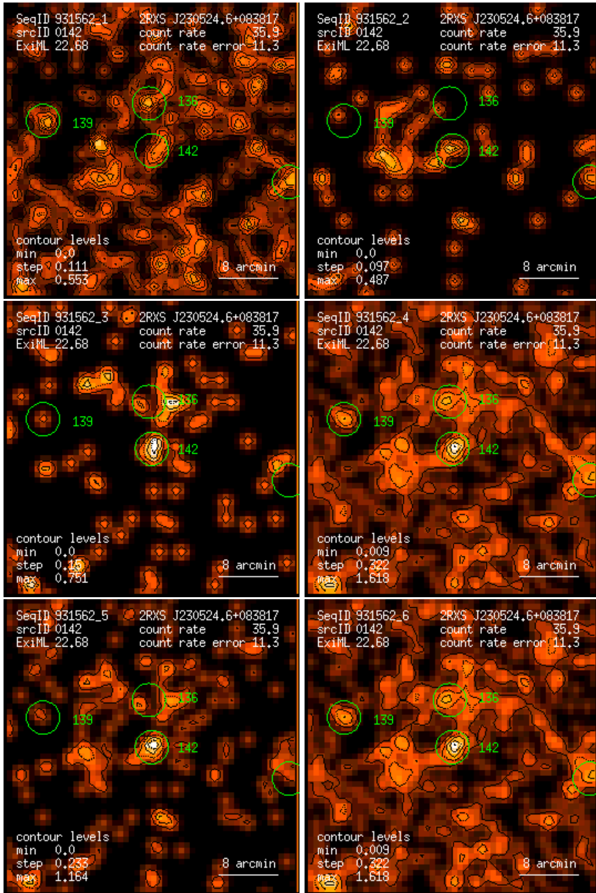
Figure 142: RASS 931562: detection 0142: band rate images, Gaussian filter: (1) PSPC channels 11 – 41, (2) 52 – 90, (3) 91 – 201, (4) 11 – 235, (5) 52 – 201, (6) 11 – 201. Broad band rates in counts/ks. Band rate contour levels in counts/ks/arcmin 2 .
