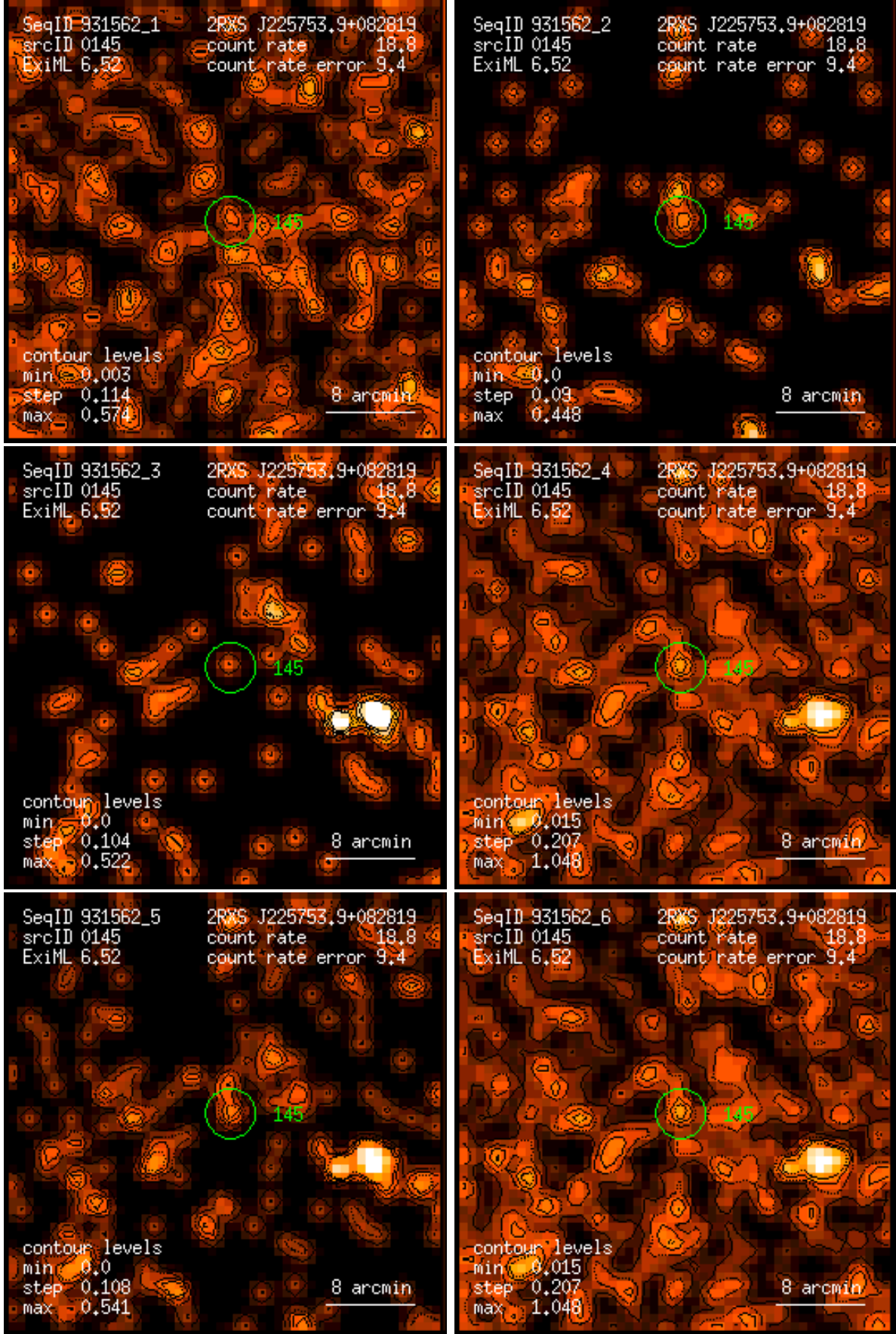
Figure 145: RASS 931562: detection 0145: band rate images, Gaussian filter: (1) PSPC channels 11 – 41, (2) 52 – 90, (3) 91 – 201, (4) 11 – 235, (5) 52 – 201, (6) 11 – 201. Broad band rates in counts/ks. Band rate contour levels in counts/ks/arcmin 2 .
