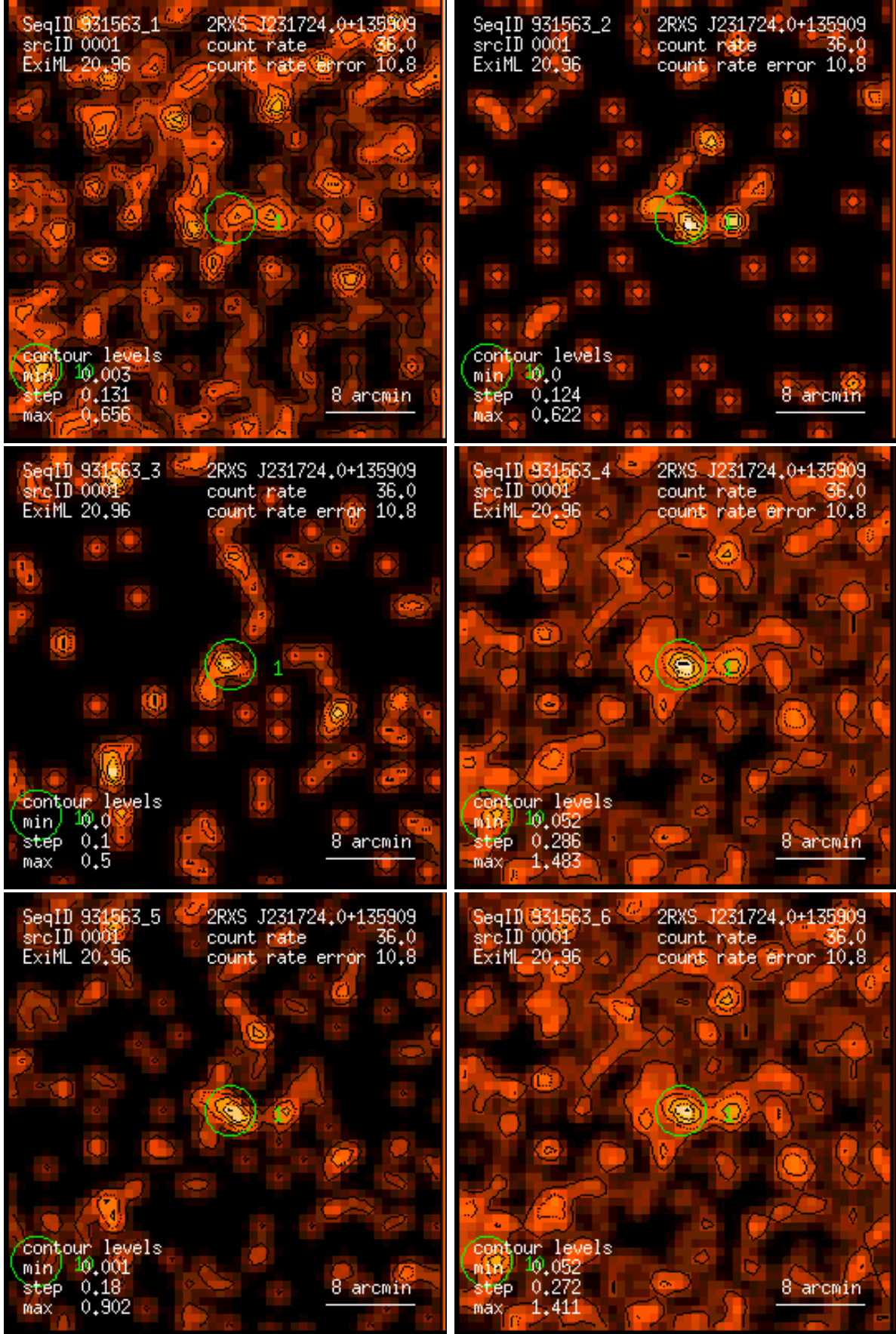
Figure 1: RASS 931563: detection 0001: band rate images, Gaussian filter: (1) PSPC channels 11 – 41, (2) 52 – 90, (3) 91 – 201, (4) 11 – 235, (5) 52 – 201, (6) 11 – 201. Broad band rates in counts/ks. Band rate contour levels in counts/ks/arcmin 2 .
