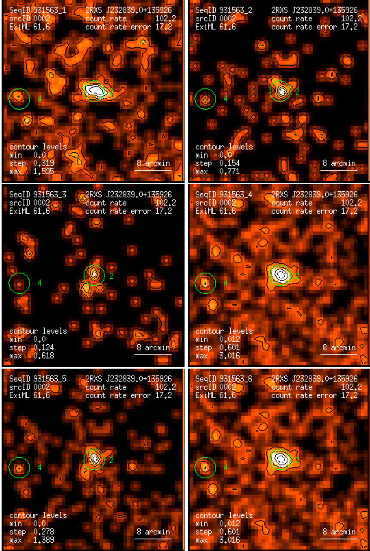
Figure 2: RASS 931563: detection 0002: band rate images, Gaussian filter: (1) PSPC channels 11 – 41, (2) 52 – 90, (3) 91 – 201, (4) 11 – 235, (5) 52 – 201, (6) 11 – 201. Broad band rates in counts/ks. Band rate contour levels in counts/ks/arcmin 2 .
