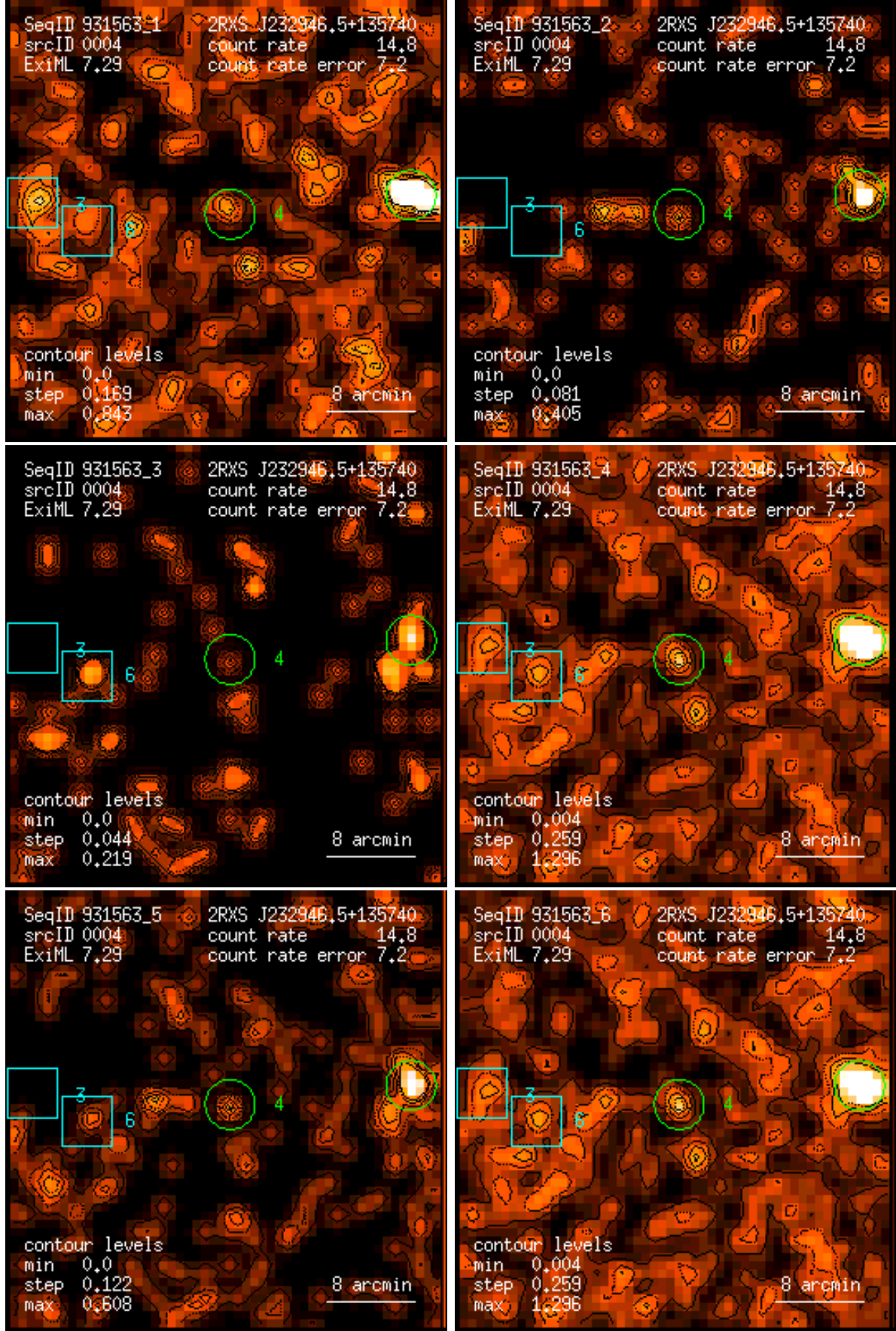
Figure 4: RASS 931563: detection 0004: band rate images, Gaussian filter: (1) PSPC channels 11 – 41, (2) 52 – 90, (3) 91 – 201, (4) 11 – 235, (5) 52 – 201, (6) 11 – 201. Broad band rates in counts/ks. Band rate contour levels in counts/ks/arcmin 2 .
