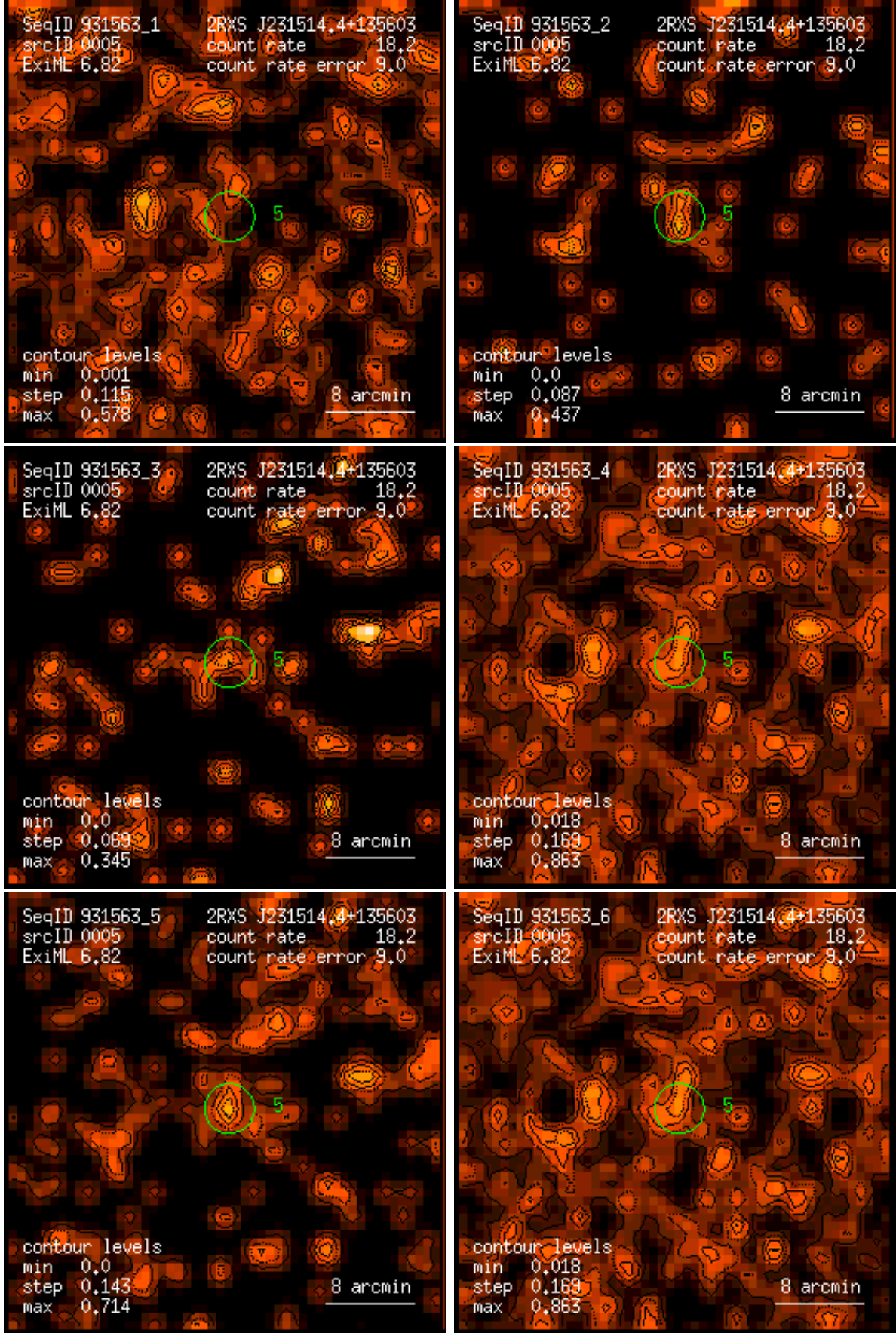
Figure 5: RASS 931563: detection 0005: band rate images, Gaussian filter: (1) PSPC channels 11 – 41, (2) 52 – 90, (3) 91 – 201, (4) 11 – 235, (5) 52 – 201, (6) 11 – 201. Broad band rates in counts/ks. Band rate contour levels in counts/ks/arcmin 2 .
