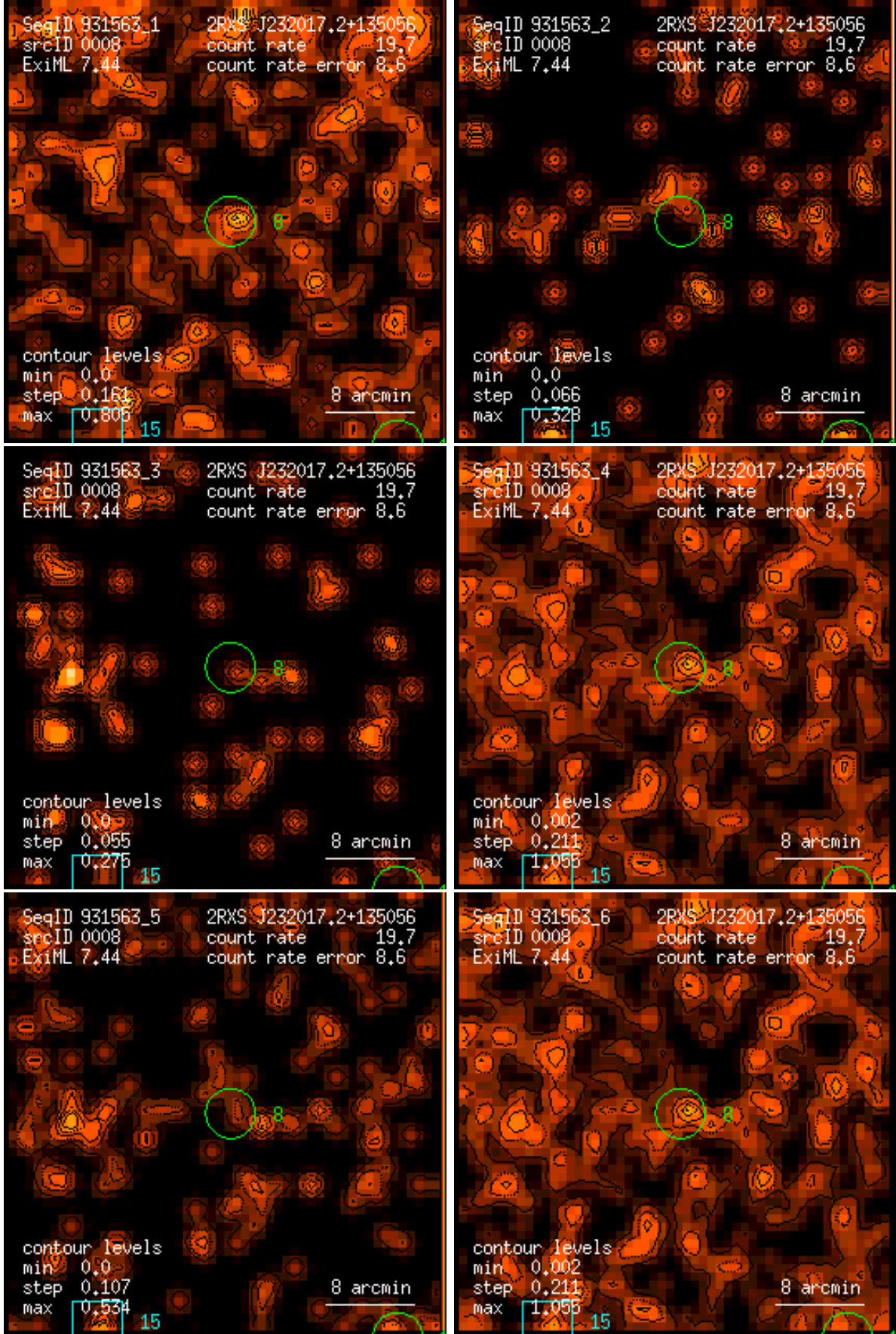
Figure 8: RASS 931563: detection 0008: band rate images, Gaussian filter: (1) PSPC channels 11 – 41, (2) 52 – 90, (3) 91 – 201, (4) 11 – 235, (5) 52 – 201, (6) 11 – 201. Broad band rates in counts/ks. Band rate contour levels in counts/ks/arcmin 2 .
