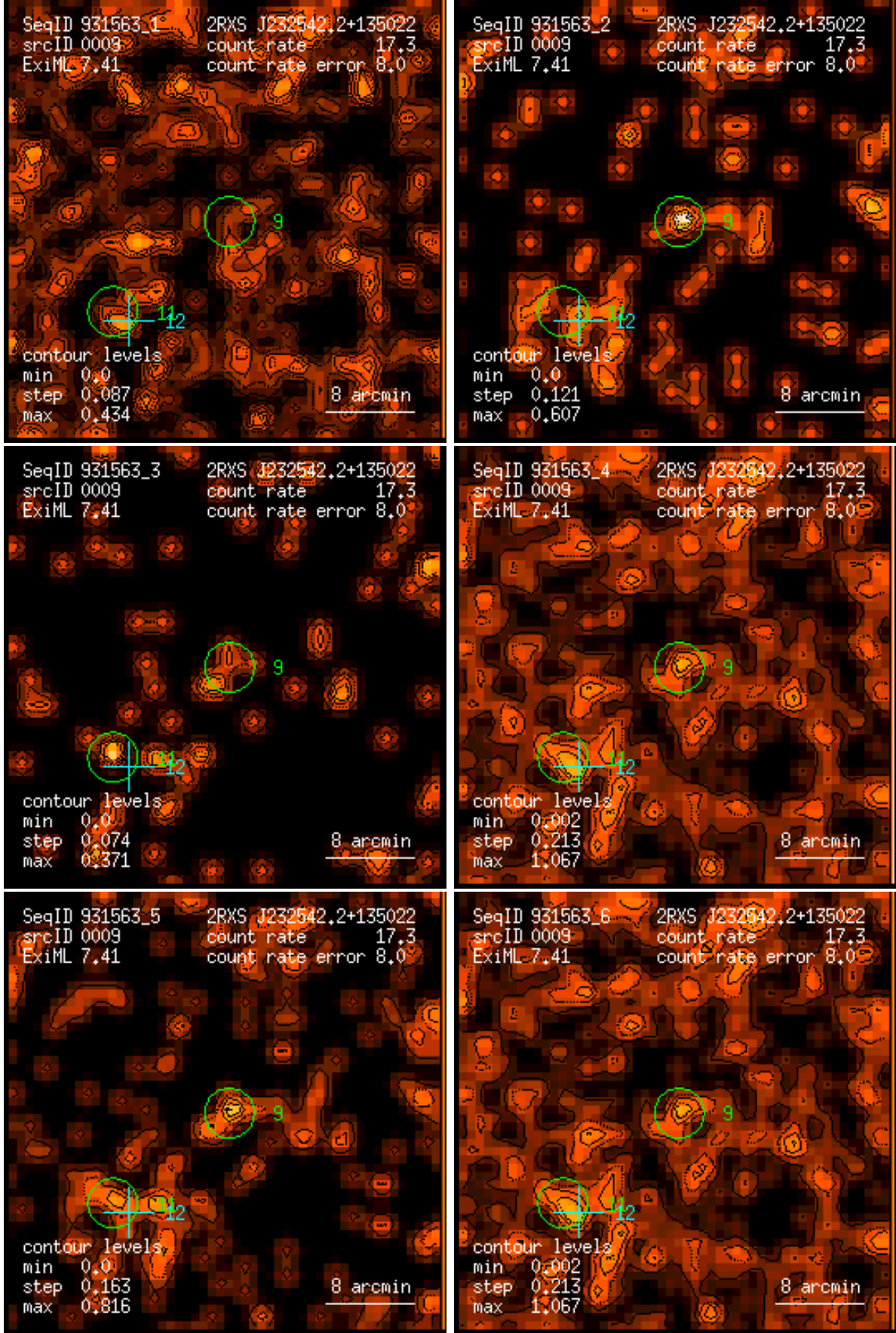
Figure 9: RASS 931563: detection 0009: band rate images, Gaussian filter: (1) PSPC channels 11 – 41, (2) 52 – 90, (3) 91 – 201, (4) 11 – 235, (5) 52 – 201, (6) 11 – 201. Broad band rates in counts/ks. Band rate contour levels in counts/ks/arcmin 2 .
