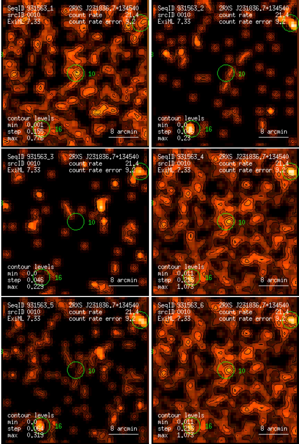
Figure 10: RASS 931563: detection 0010: band rate images, Gaussian filter: (1) PSPC channels 11 – 41, (2) 52 – 90, (3) 91 – 201, (4) 11 – 235, (5) 52 – 201, (6) 11 – 201. Broad band rates in counts/ks. Band rate contour levels in counts/ks/arcmin 2 .
