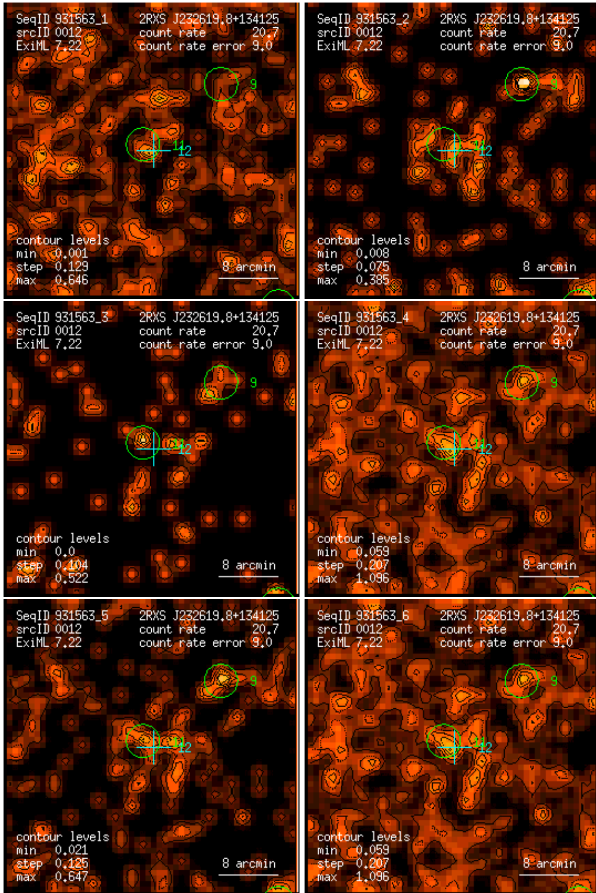
Figure 12: RASS 931563: detection 0012: band rate images, Gaussian filter: (1) PSPC channels 11 – 41, (2) 52 – 90, (3) 91 – 201, (4) 11 – 235, (5) 52 – 201, (6) 11 – 201. Broad band rates in counts/ks. Band rate contour levels in counts/ks/arcmin 2 .
