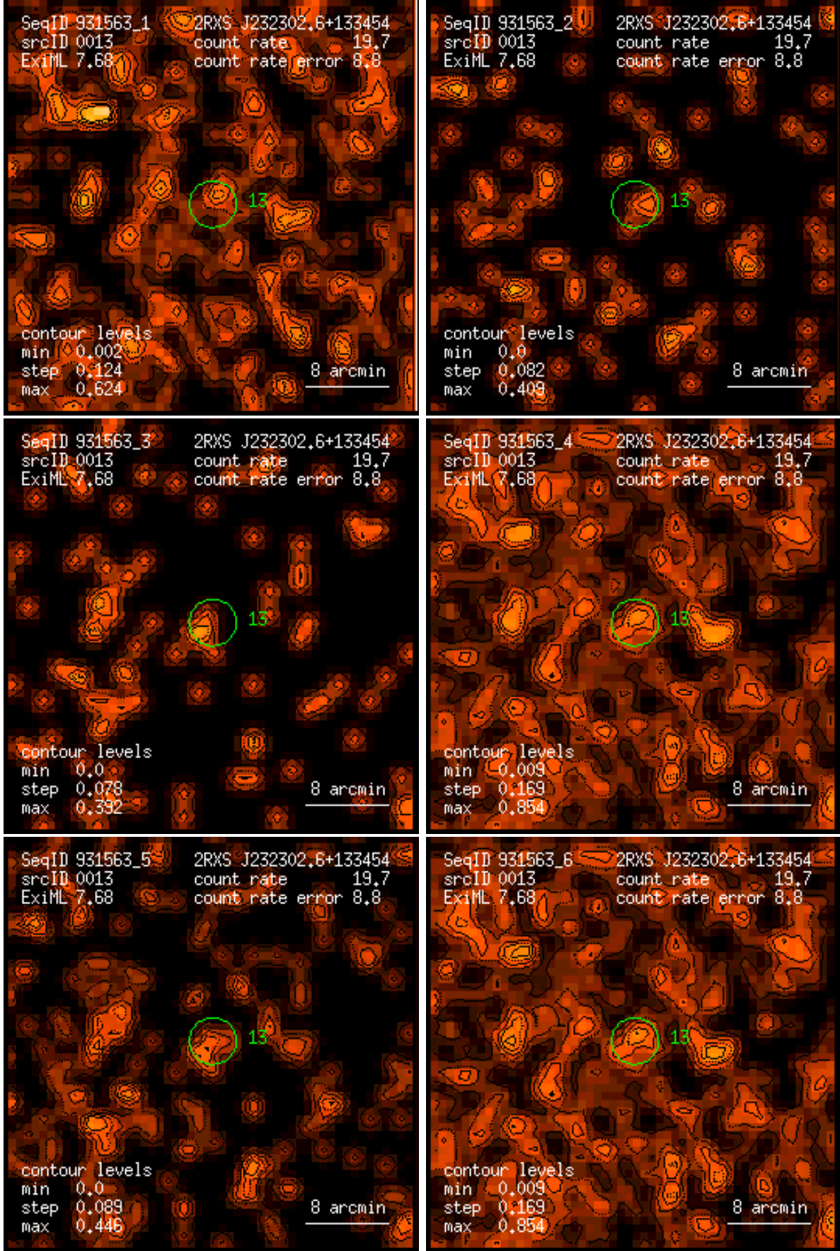
Figure 13: RASS 931563: detection 0013: band rate images, Gaussian filter: (1) PSPC channels 11 – 41, (2) 52 – 90, (3) 91 – 201, (4) 11 – 235, (5) 52 – 201, (6) 11 – 201. Broad band rates in counts/ks. Band rate contour levels in counts/ks/arcmin 2 .
