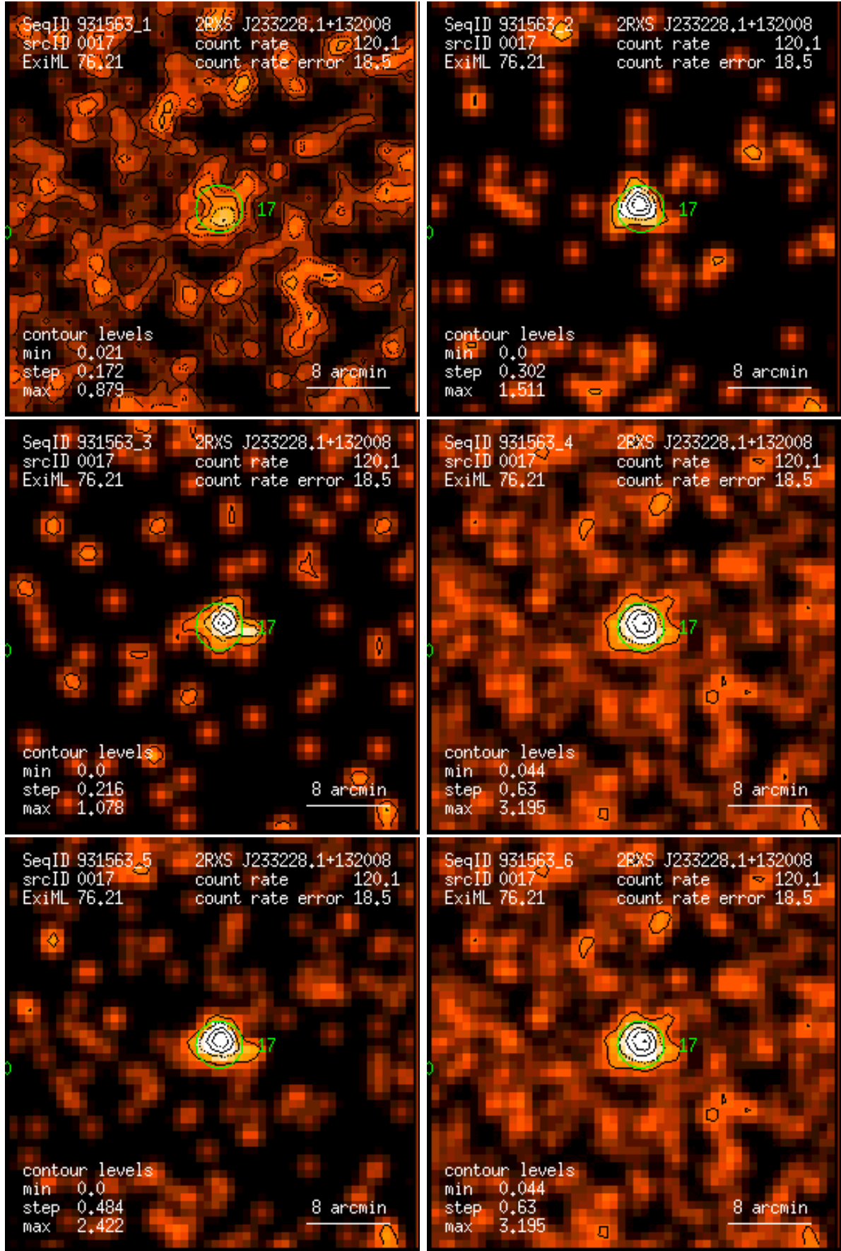
Figure 17: RASS 931563: detection 0017: band rate images, Gaussian filter: (1) PSPC channels 11 – 41, (2) 52 – 90, (3) 91 – 201, (4) 11 – 235, (5) 52 – 201, (6) 11 – 201. Broad band rates in counts/ks. Band rate contour levels in counts/ks/arcmin 2 .
