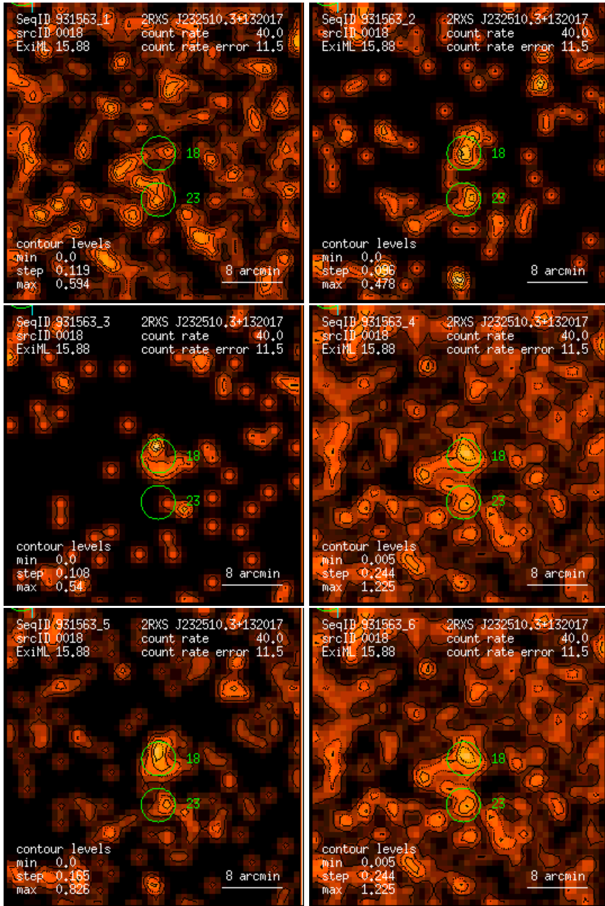
Figure 18: RASS 931563: detection 0018: band rate images, Gaussian filter: (1) PSPC channels 11 – 41, (2) 52 – 90, (3) 91 – 201, (4) 11 – 235, (5) 52 – 201, (6) 11 – 201. Broad band rates in counts/ks. Band rate contour levels in counts/ks/arcmin 2 .
