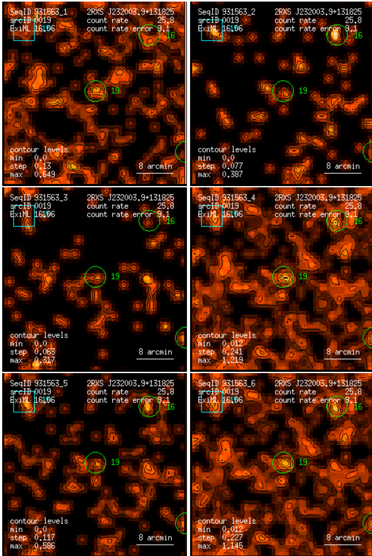
Figure 19: RASS 931563: detection 0019: band rate images, Gaussian filter: (1) PSPC channels 11 – 41, (2) 52 – 90, (3) 91 – 201, (4) 11 – 235, (5) 52 – 201, (6) 11 – 201. Broad band rates in counts/ks. Band rate contour levels in counts/ks/arcmin 2 .
