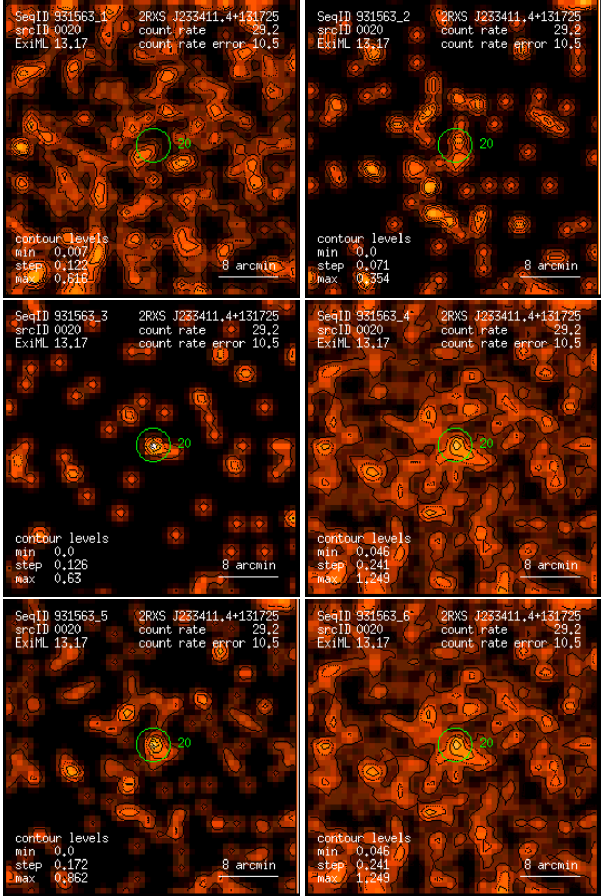
Figure 20: RASS 931563: detection 0020: band rate images, Gaussian filter: (1) PSPC channels 11 – 41, (2) 52 – 90, (3) 91 – 201, (4) 11 – 235, (5) 52 – 201, (6) 11 – 201. Broad band rates in counts/ks. Band rate contour levels in counts/ks/arcmin 2 .
