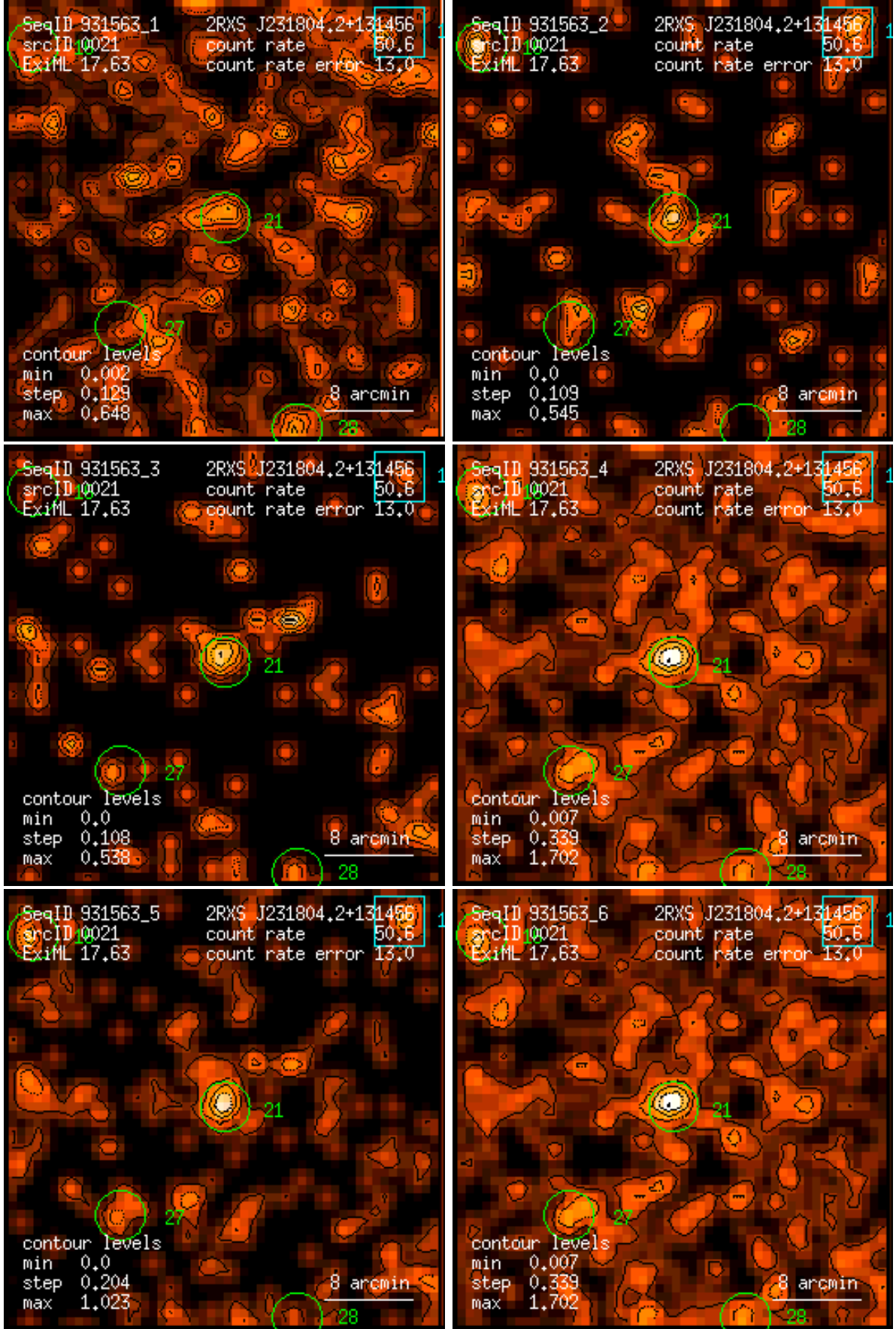
Figure 21: RASS 931563: detection 0021: band rate images, Gaussian filter: (1) PSPC channels 11 – 41, (2) 52 – 90, (3) 91 – 201, (4) 11 – 235, (5) 52 – 201, (6) 11 – 201. Broad band rates in counts/ks. Band rate contour levels in counts/ks/arcmin 2 .
