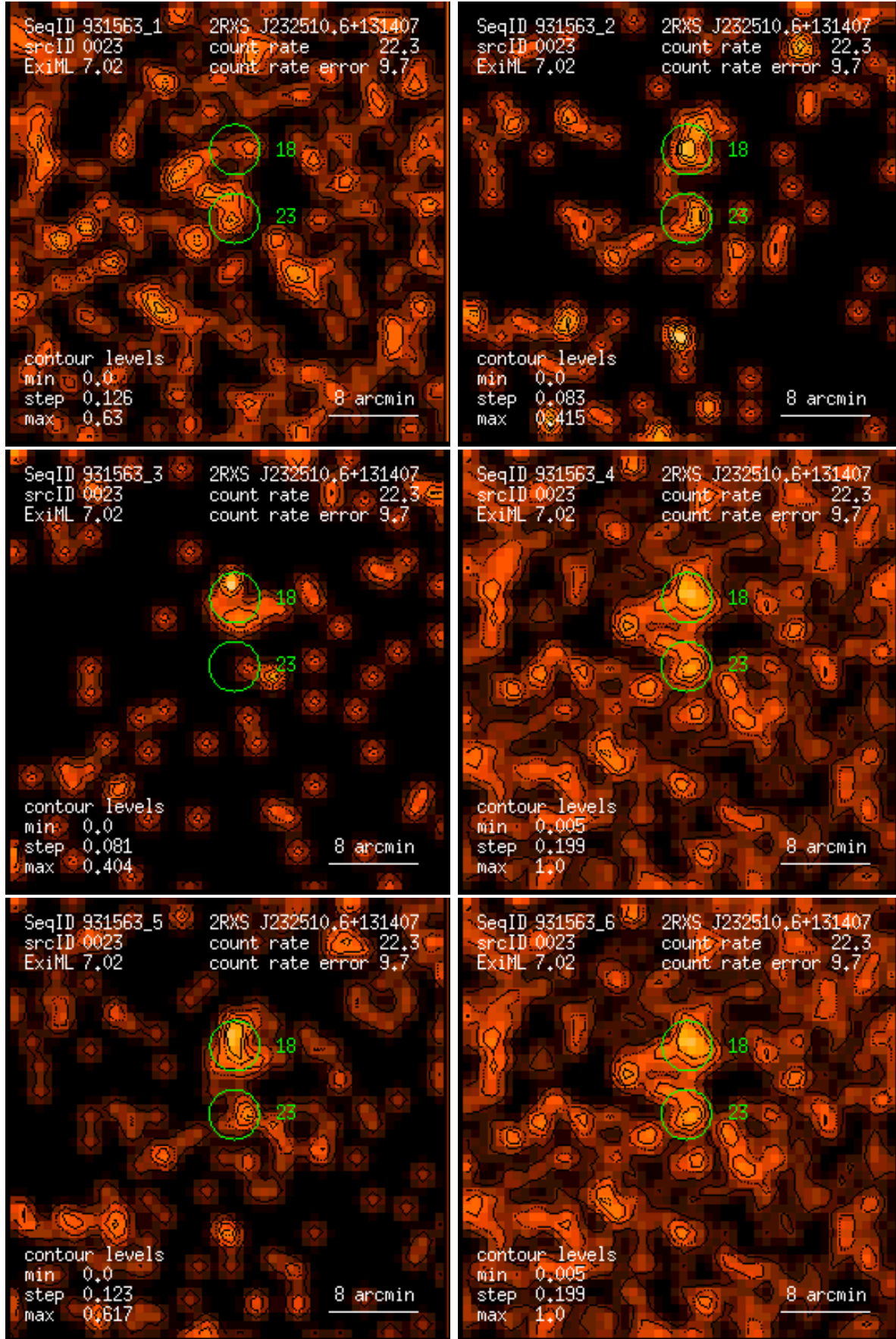
Figure 23: RASS 931563: detection 0023: band rate images, Gaussian filter: (1) PSPC channels 11 – 41, (2) 52 – 90, (3) 91 – 201, (4) 11 – 235, (5) 52 – 201, (6) 11 – 201. Broad band rates in counts/ks. Band rate contour levels in counts/ks/arcmin 2 .
