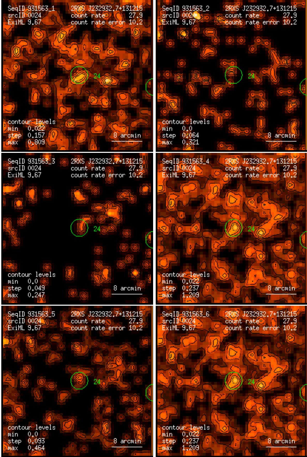
Figure 24: RASS 931563: detection 0024: band rate images, Gaussian filter: (1) PSPC channels 11 – 41, (2) 52 – 90, (3) 91 – 201, (4) 11 – 235, (5) 52 – 201, (6) 11 – 201. Broad band rates in counts/ks. Band rate contour levels in counts/ks/arcmin 2 .
