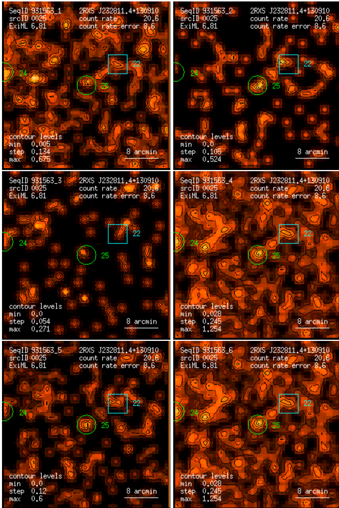
Figure 25: RASS 931563: detection 0025: band rate images, Gaussian filter: (1) PSPC channels 11 – 41, (2) 52 – 90, (3) 91 – 201, (4) 11 – 235, (5) 52 – 201, (6) 11 – 201. Broad band rates in counts/ks. Band rate contour levels in counts/ks/arcmin 2 .
