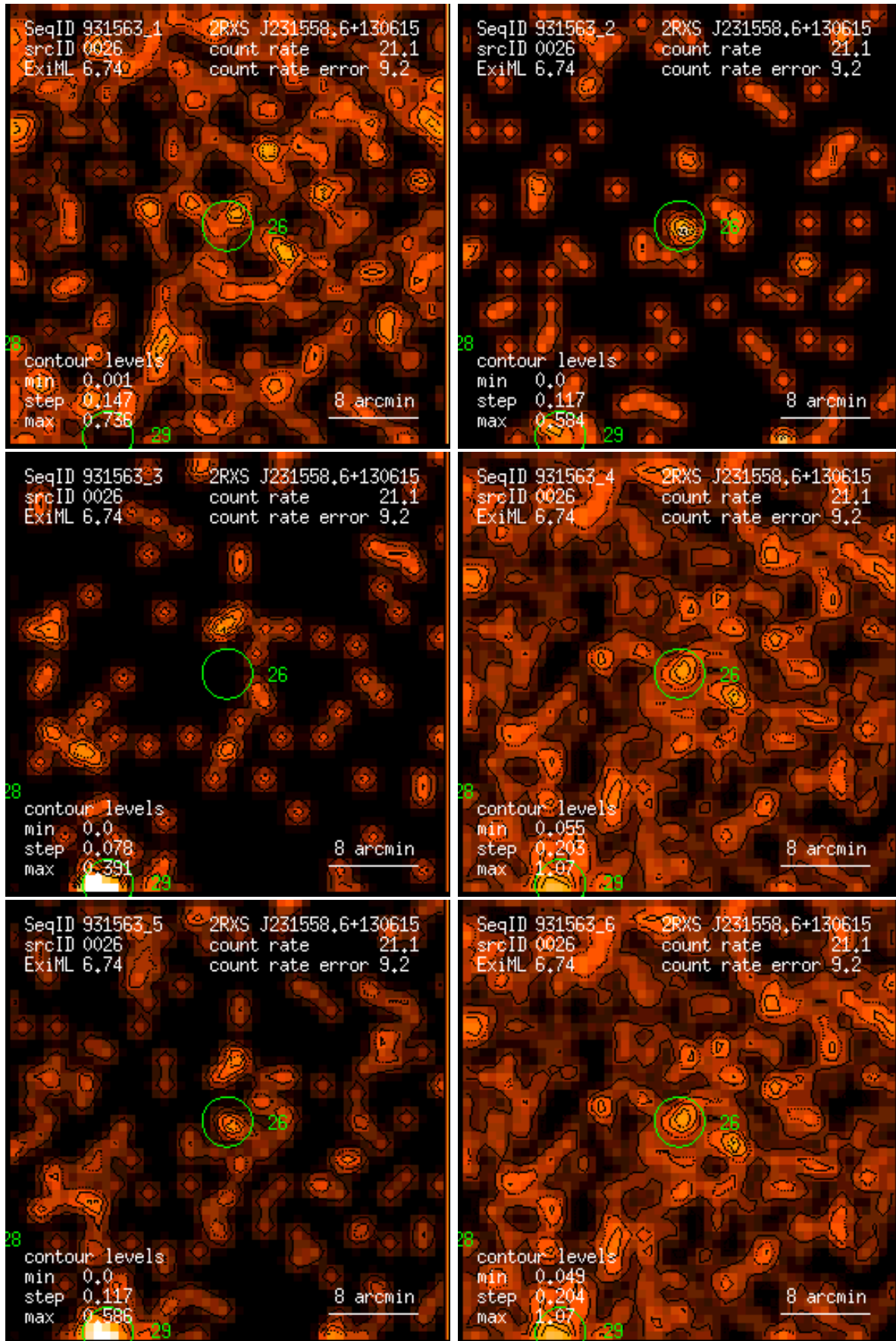
Figure 26: RASS 931563: detection 0026: band rate images, Gaussian filter: (1) PSPC channels 11 – 41, (2) 52 – 90, (3) 91 – 201, (4) 11 – 235, (5) 52 – 201, (6) 11 – 201. Broad band rates in counts/ks. Band rate contour levels in counts/ks/arcmin 2 .
