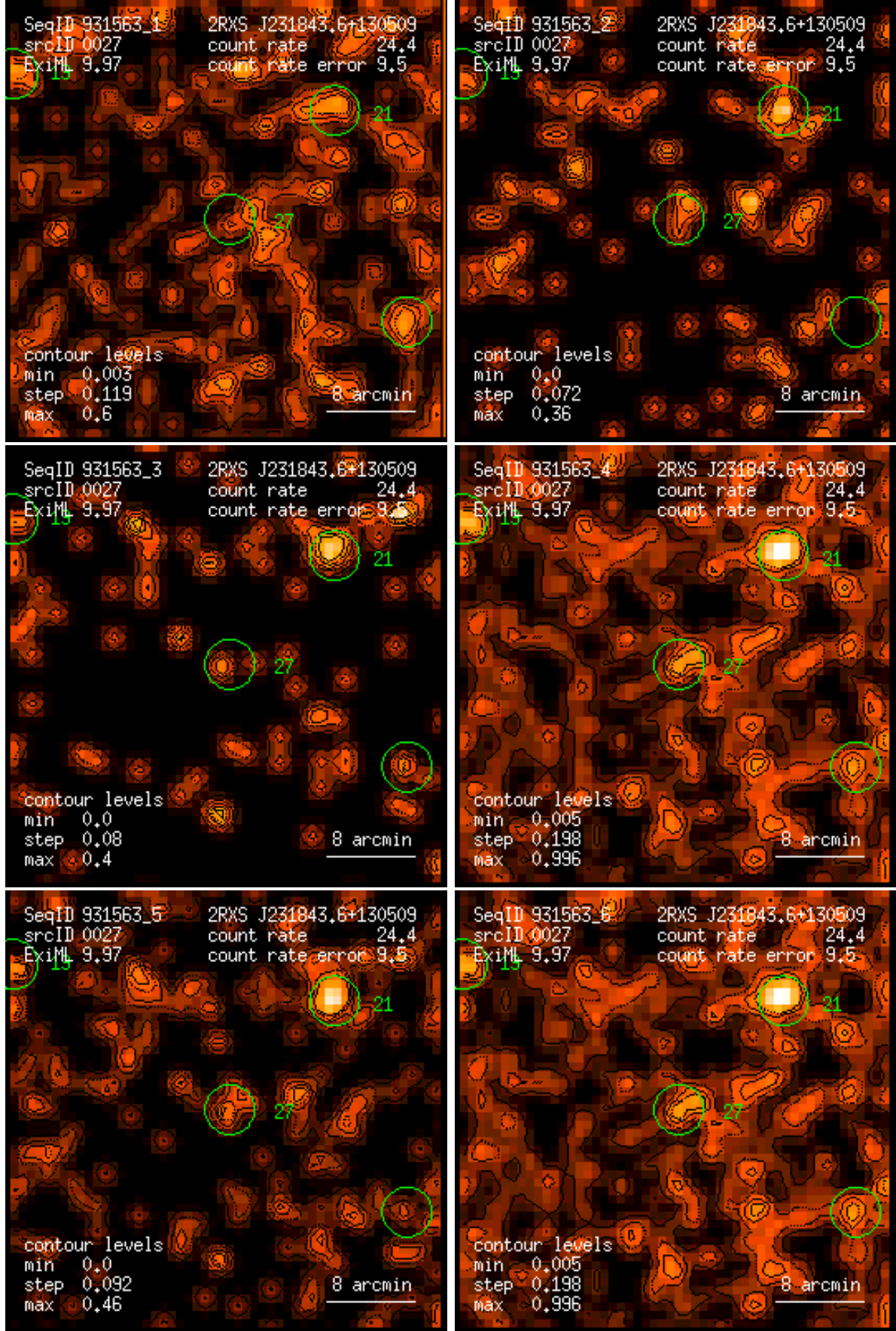
Figure 27: RASS 931563: detection 0027: band rate images, Gaussian filter: (1) PSPC channels 11 – 41, (2) 52 – 90, (3) 91 – 201, (4) 11 – 235, (5) 52 – 201, (6) 11 – 201. Broad band rates in counts/ks. Band rate contour levels in counts/ks/arcmin 2 .
