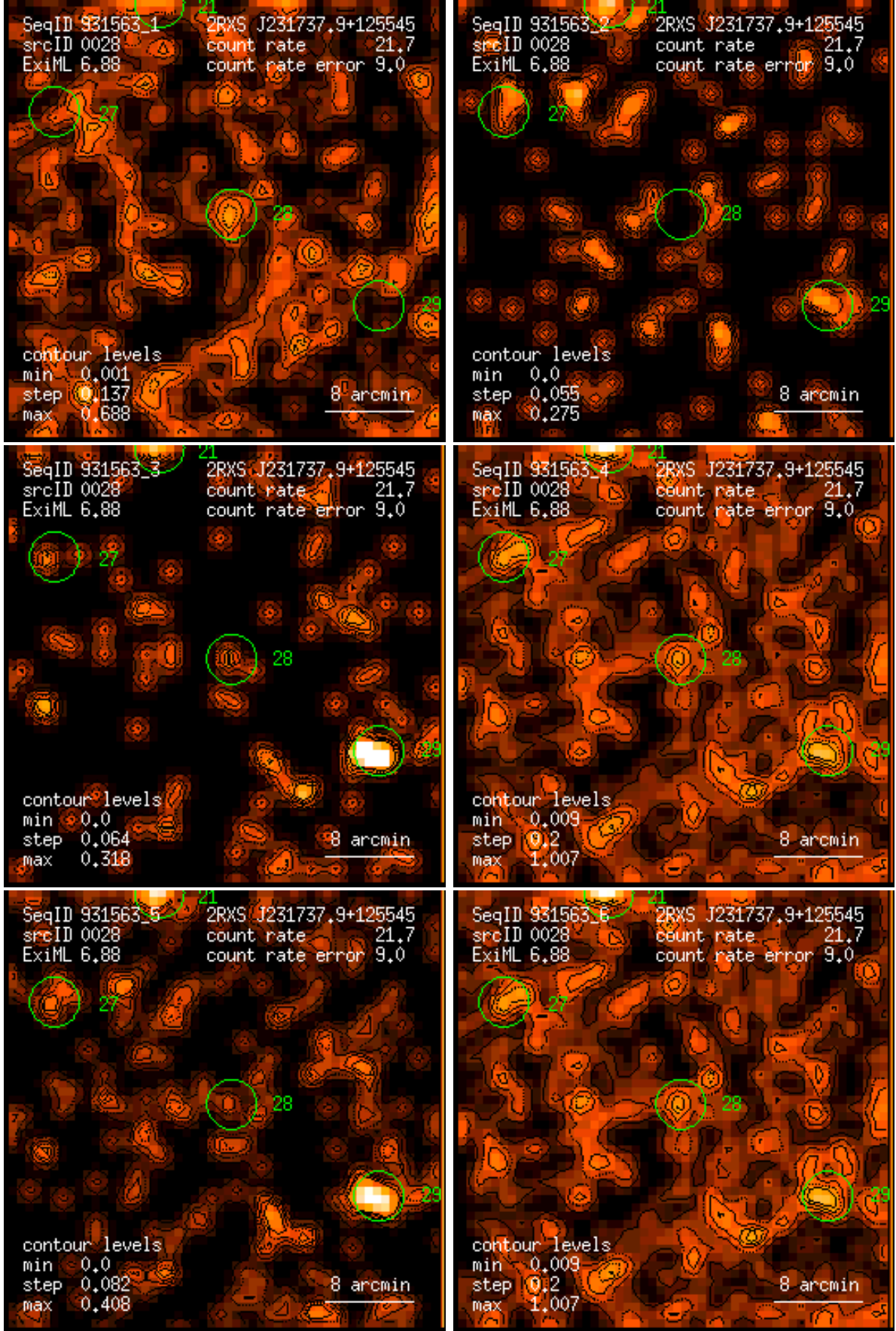
Figure 28: RASS 931563: detection 0028: band rate images, Gaussian filter: (1) PSPC channels 11 – 41, (2) 52 – 90, (3) 91 – 201, (4) 11 – 235, (5) 52 – 201, (6) 11 – 201. Broad band rates in counts/ks. Band rate contour levels in counts/ks/arcmin 2 .
