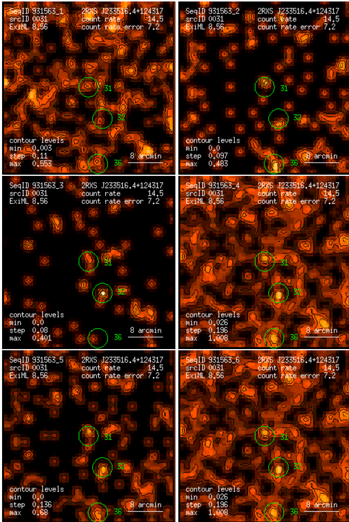
Figure 31: RASS 931563: detection 0031: band rate images, Gaussian filter: (1) PSPC channels 11 – 41, (2) 52 – 90, (3) 91 – 201, (4) 11 – 235, (5) 52 – 201, (6) 11 – 201. Broad band rates in counts/ks. Band rate contour levels in counts/ks/arcmin 2 .
