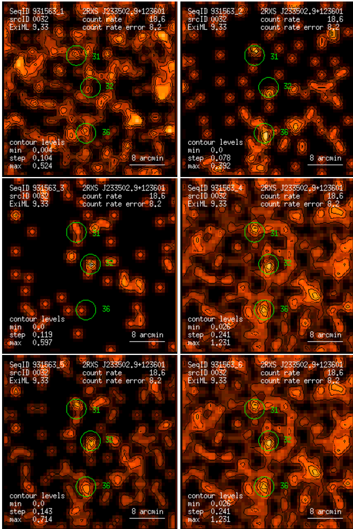
Figure 32: RASS 931563: detection 0032: band rate images, Gaussian filter: (1) PSPC channels 11 – 41, (2) 52 – 90, (3) 91 – 201, (4) 11 – 235, (5) 52 – 201, (6) 11 – 201. Broad band rates in counts/ks. Band rate contour levels in counts/ks/arcmin 2 .
