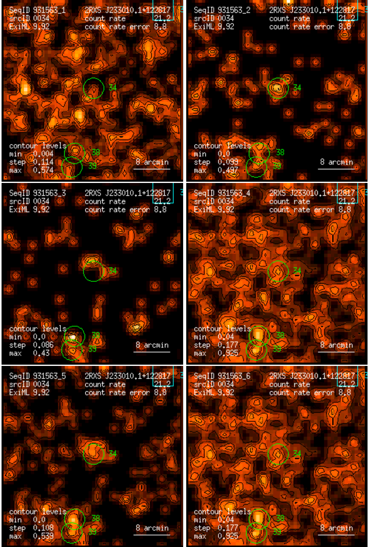
Figure 34: RASS 931563: detection 0034: band rate images, Gaussian filter: (1) PSPC channels 11 – 41, (2) 52 – 90, (3) 91 – 201, (4) 11 – 235, (5) 52 – 201, (6) 11 – 201. Broad band rates in counts/ks. Band rate contour levels in counts/ks/arcmin 2 .
