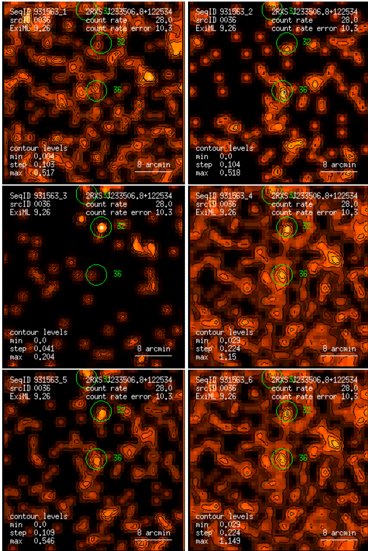
Figure 36: RASS 931563: detection 0036: band rate images, Gaussian filter: (1) PSPC channels 11 – 41, (2) 52 – 90, (3) 91 – 201, (4) 11 – 235, (5) 52 – 201, (6) 11 – 201. Broad band rates in counts/ks. Band rate contour levels in counts/ks/arcmin 2 .
