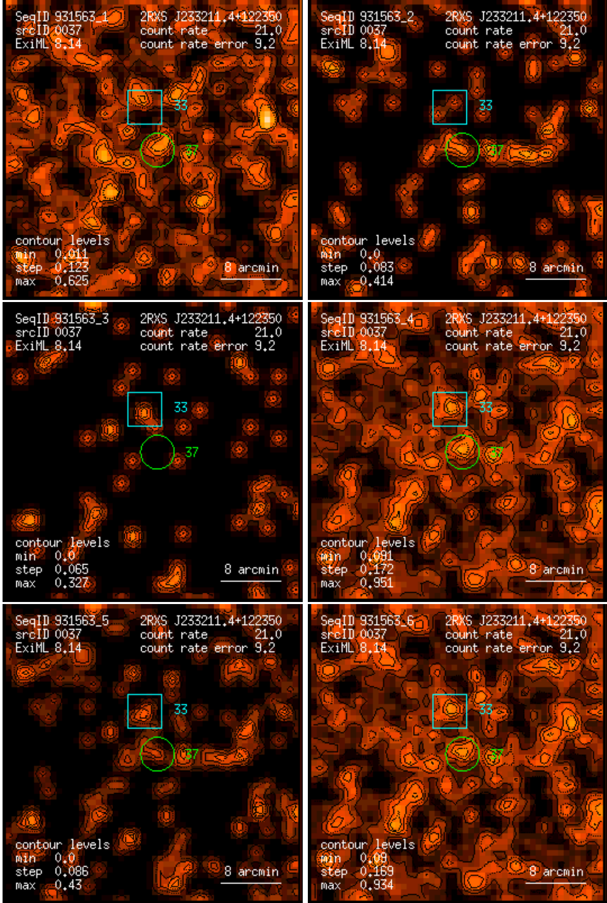
Figure 37: RASS 931563: detection 0037: band rate images, Gaussian filter: (1) PSPC channels 11 – 41, (2) 52 – 90, (3) 91 – 201, (4) 11 – 235, (5) 52 – 201, (6) 11 – 201. Broad band rates in counts/ks. Band rate contour levels in counts/ks/arcmin 2 .
