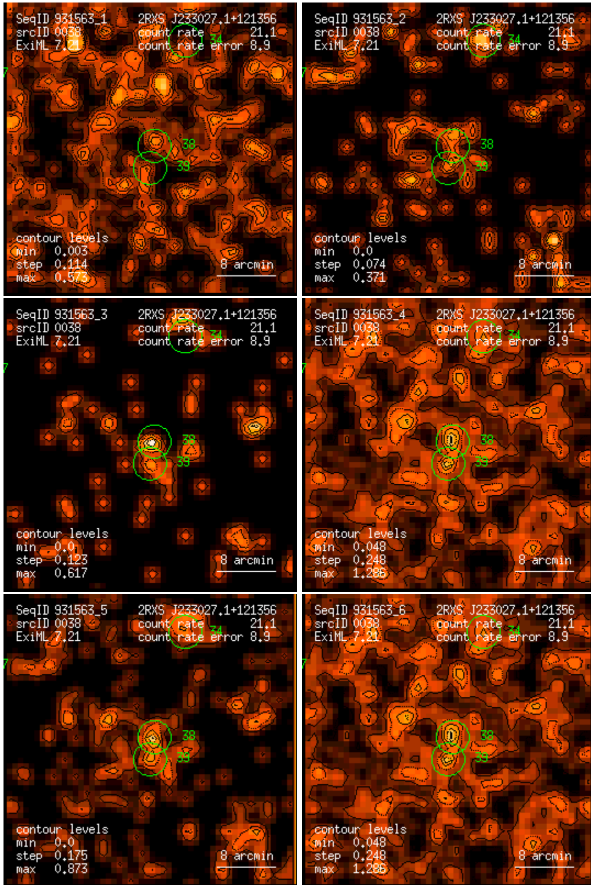
Figure 38: RASS 931563: detection 0038: band rate images, Gaussian filter: (1) PSPC channels 11 – 41, (2) 52 – 90, (3) 91 – 201, (4) 11 – 235, (5) 52 – 201, (6) 11 – 201. Broad band rates in counts/ks. Band rate contour levels in counts/ks/arcmin 2 .
