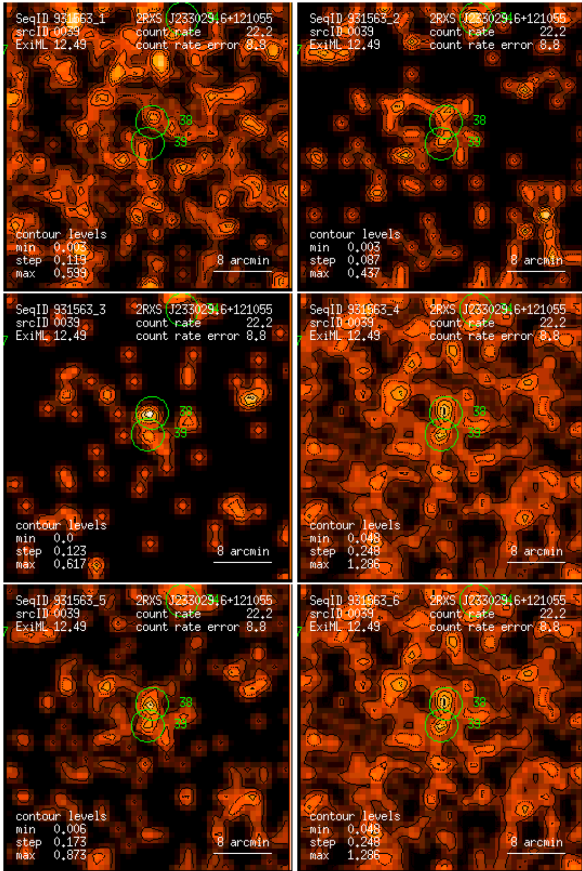
Figure 39: RASS 931563: detection 0039: band rate images, Gaussian filter: (1) PSPC channels 11 – 41, (2) 52 – 90, (3) 91 – 201, (4) 11 – 235, (5) 52 – 201, (6) 11 – 201. Broad band rates in counts/ks. Band rate contour levels in counts/ks/arcmin 2 .
