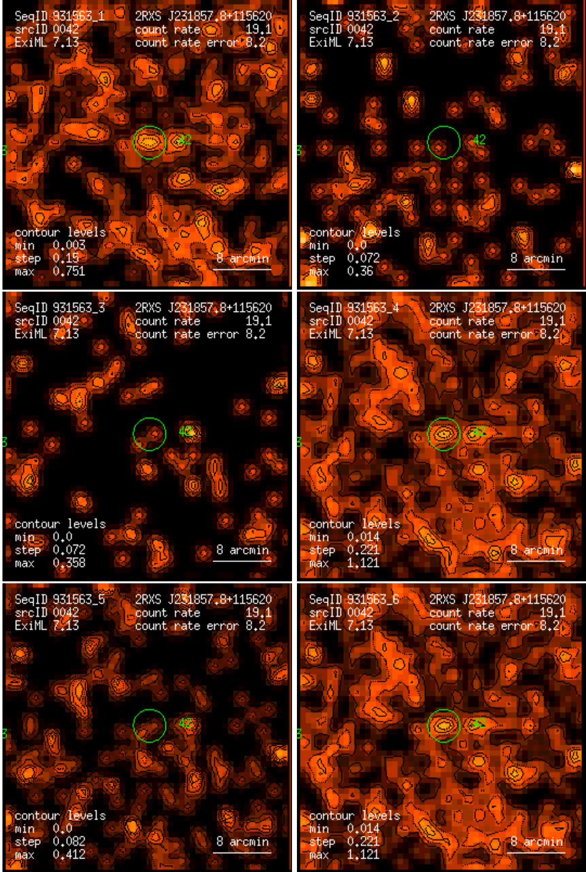
Figure 42: RASS 931563: detection 0042: band rate images, Gaussian filter: (1) PSPC channels 11 – 41, (2) 52 – 90, (3) 91 – 201, (4) 11 – 235, (5) 52 – 201, (6) 11 – 201. Broad band rates in counts/ks. Band rate contour levels in counts/ks/arcmin 2 .
