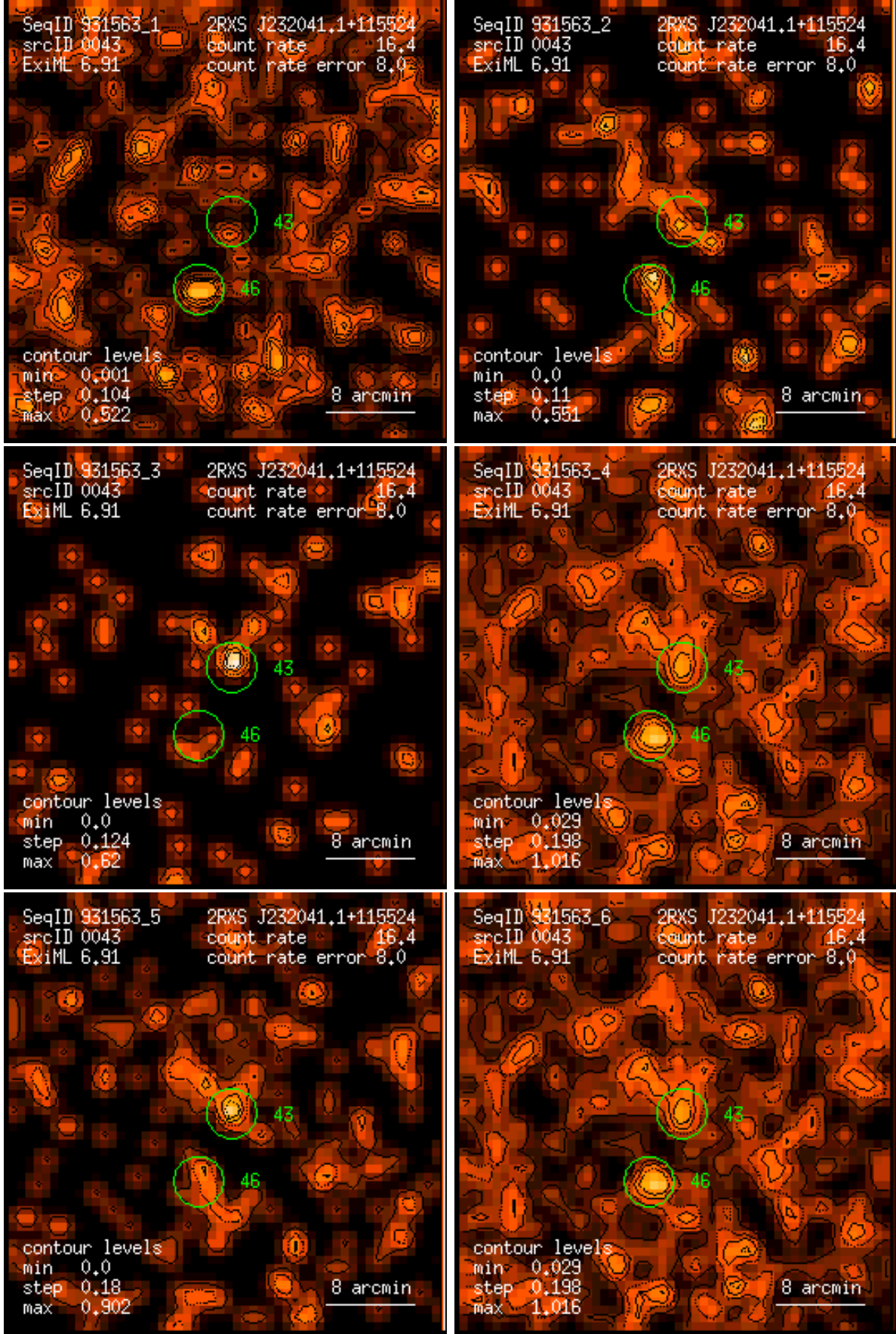
Figure 43: RASS 931563: detection 0043: band rate images, Gaussian filter: (1) PSPC channels 11 – 41, (2) 52 – 90, (3) 91 – 201, (4) 11 – 235, (5) 52 – 201, (6) 11 – 201. Broad band rates in counts/ks. Band rate contour levels in counts/ks/arcmin 2 .
