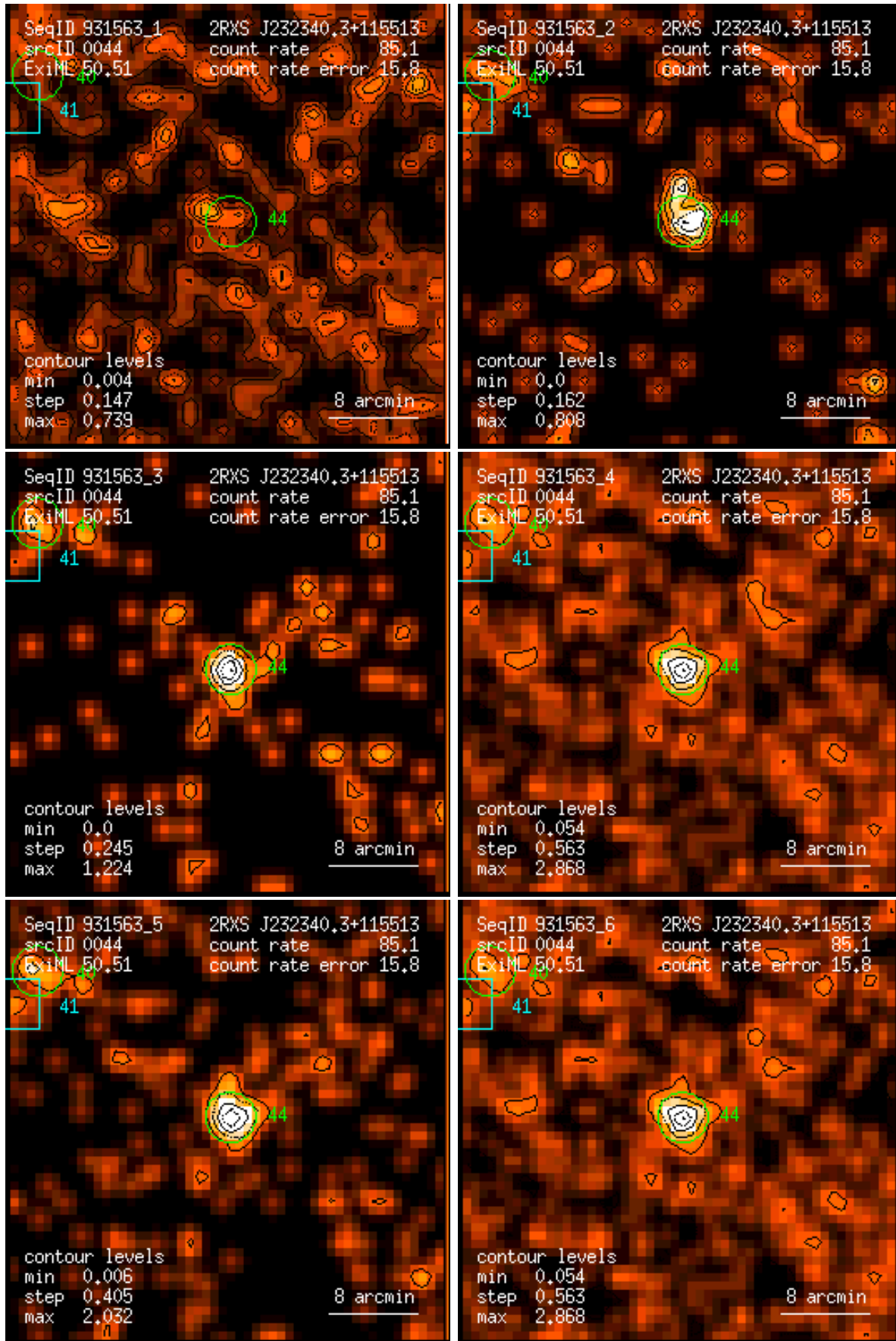
Figure 44: RASS 931563: detection 0044: band rate images, Gaussian filter: (1) PSPC channels 11 – 41, (2) 52 – 90, (3) 91 – 201, (4) 11 – 235, (5) 52 – 201, (6) 11 – 201. Broad band rates in counts/ks. Band rate contour levels in counts/ks/arcmin 2 .
