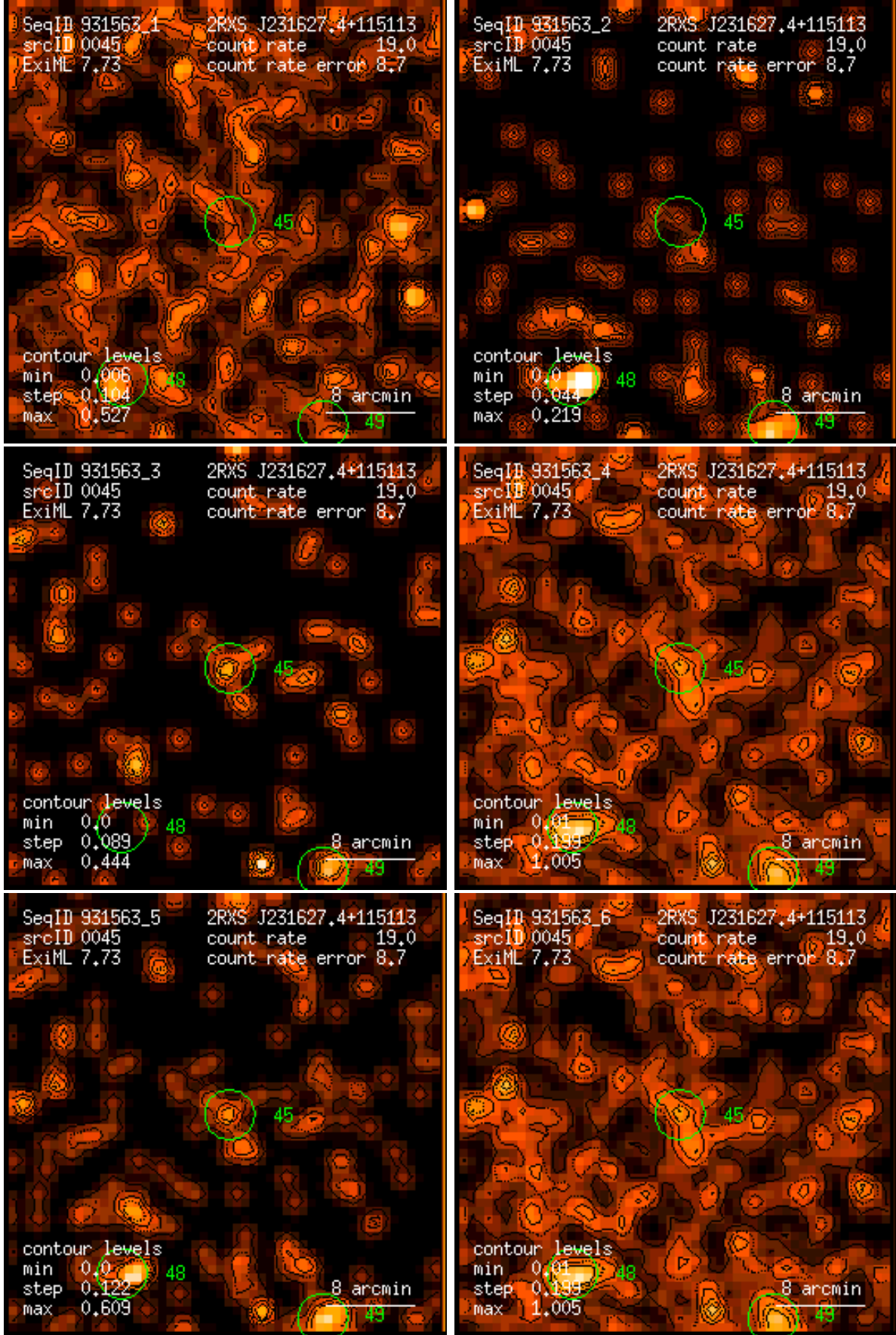
Figure 45: RASS 931563: detection 0045: band rate images, Gaussian filter: (1) PSPC channels 11 – 41, (2) 52 – 90, (3) 91 – 201, (4) 11 – 235, (5) 52 – 201, (6) 11 – 201. Broad band rates in counts/ks. Band rate contour levels in counts/ks/arcmin 2 .
