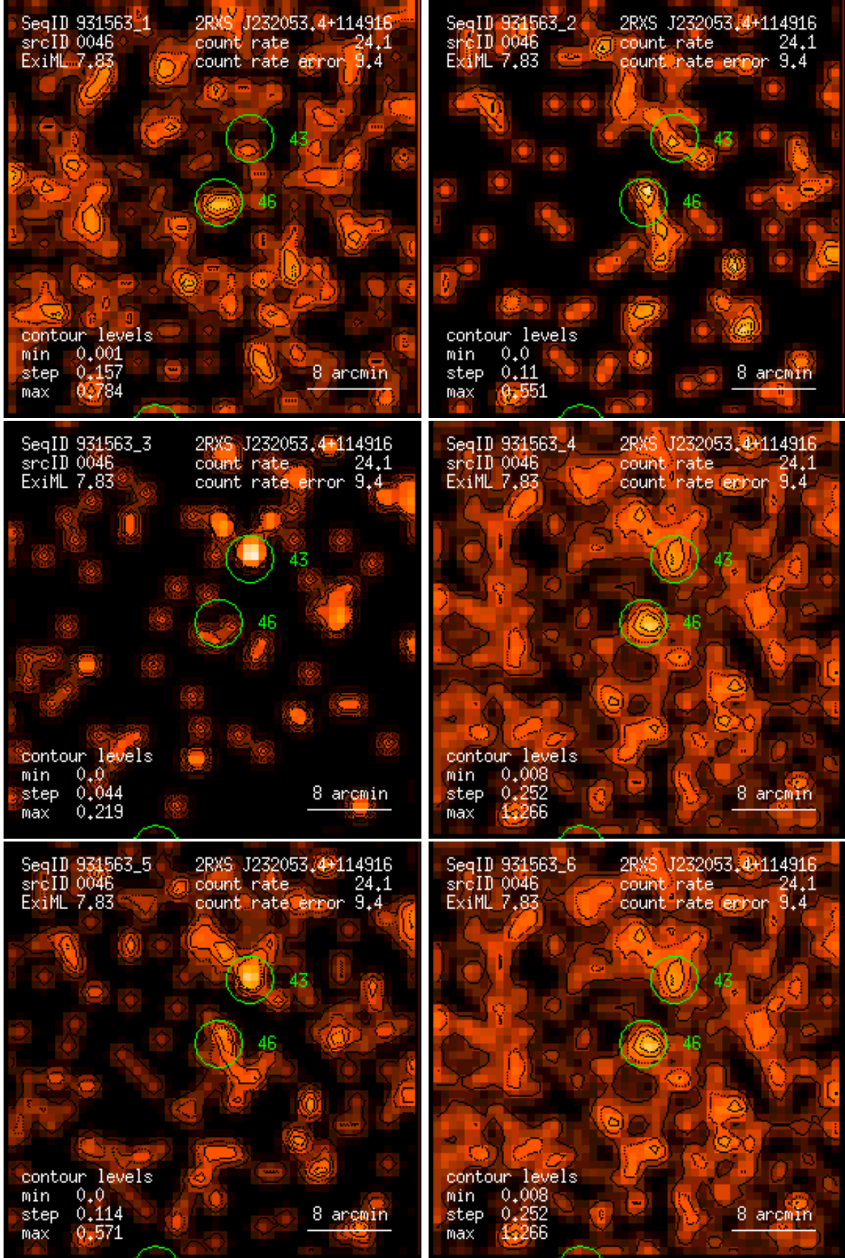
Figure 46: RASS 931563: detection 0046: band rate images, Gaussian filter: (1) PSPC channels 11 – 41, (2) 52 – 90, (3) 91 – 201, (4) 11 – 235, (5) 52 – 201, (6) 11 – 201. Broad band rates in counts/ks. Band rate contour levels in counts/ks/arcmin 2 .
