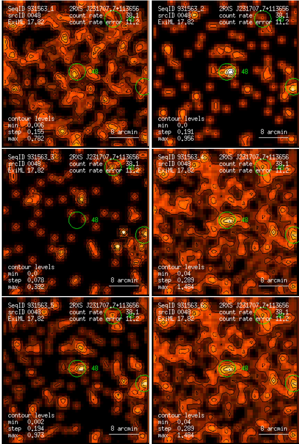
Figure 48: RASS 931563: detection 0048: band rate images, Gaussian filter: (1) PSPC channels 11 – 41, (2) 52 – 90, (3) 91 – 201, (4) 11 – 235, (5) 52 – 201, (6) 11 – 201. Broad band rates in counts/ks. Band rate contour levels in counts/ks/arcmin 2 .
