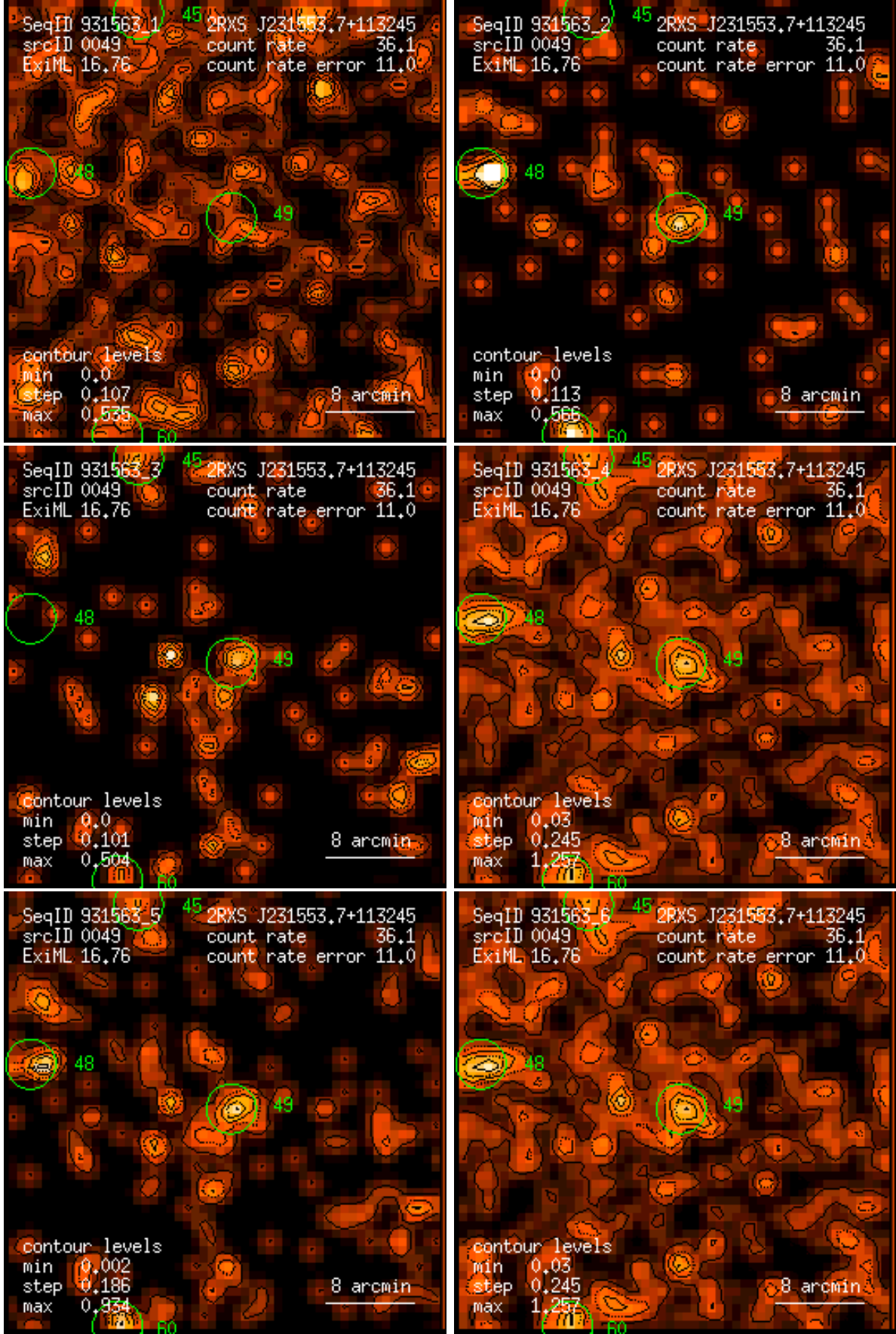
Figure 49: RASS 931563: detection 0049: band rate images, Gaussian filter: (1) PSPC channels 11 – 41, (2) 52 – 90, (3) 91 – 201, (4) 11 – 235, (5) 52 – 201, (6) 11 – 201. Broad band rates in counts/ks. Band rate contour levels in counts/ks/arcmin 2 .
