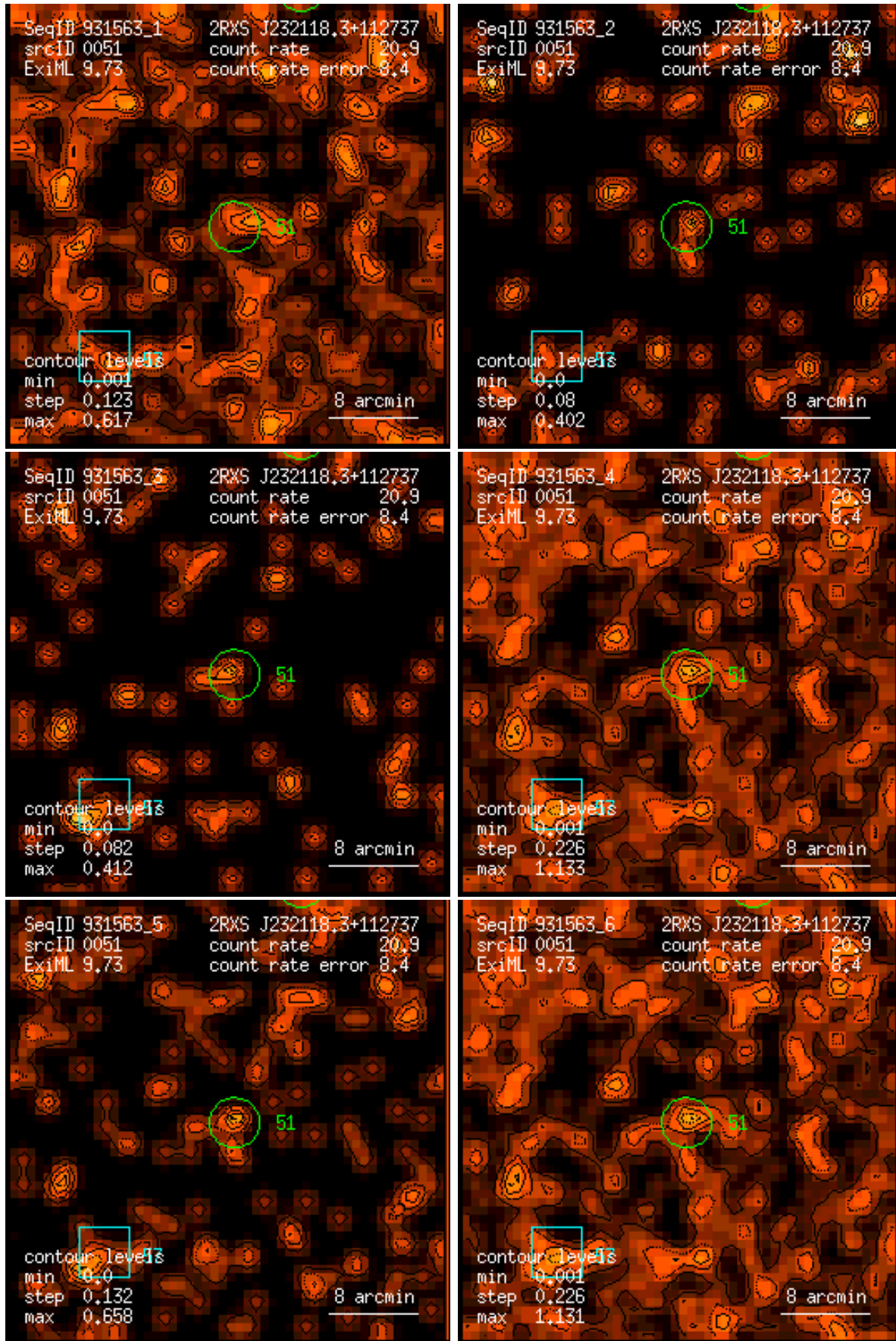
Figure 51: RASS 931563: detection 0051: band rate images, Gaussian filter: (1) PSPC channels 11 – 41, (2) 52 – 90, (3) 91 – 201, (4) 11 – 235, (5) 52 – 201, (6) 11 – 201. Broad band rates in counts/ks. Band rate contour levels in counts/ks/arcmin 2 .
