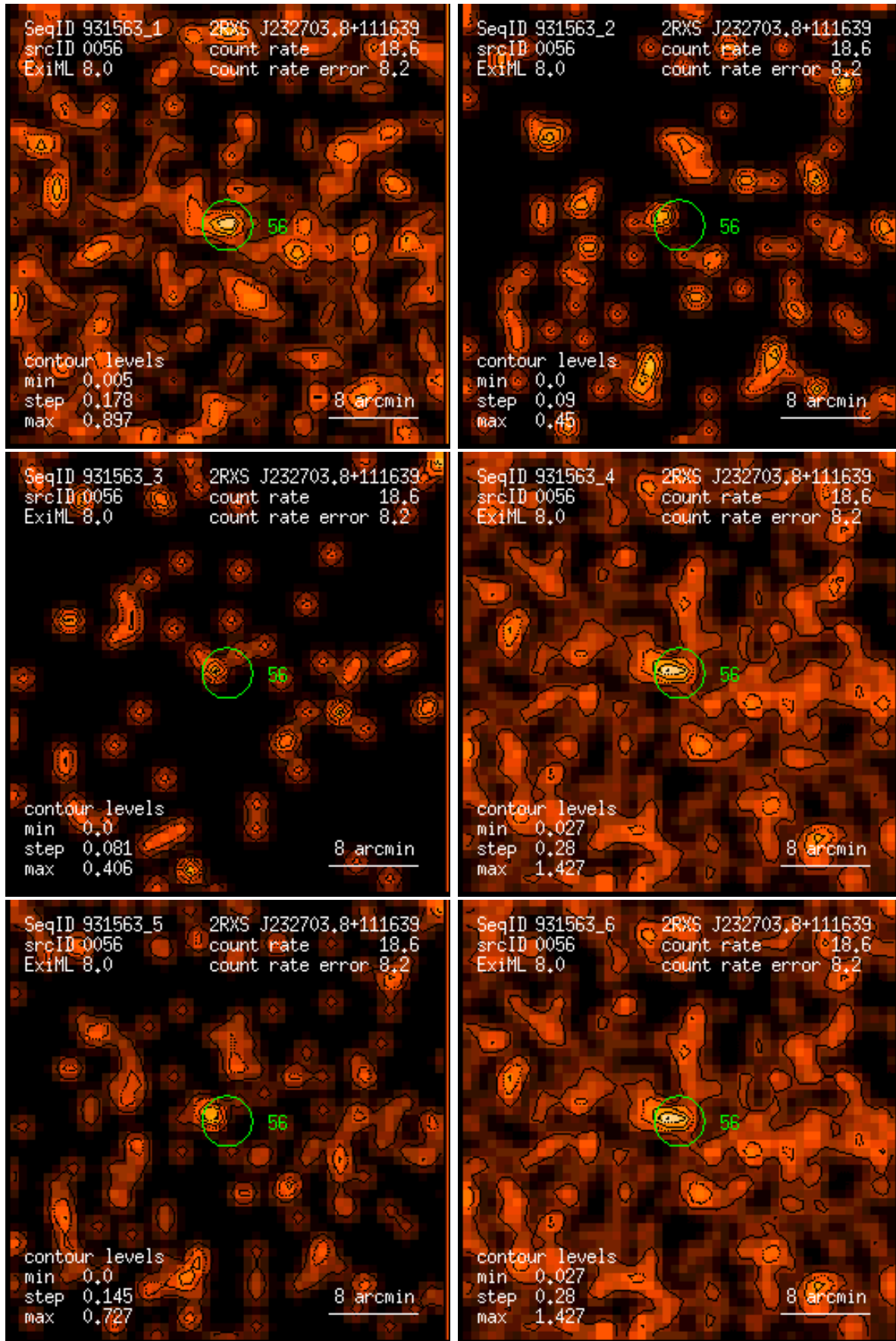
Figure 56: RASS 931563: detection 0056: band rate images, Gaussian filter: (1) PSPC channels 11 – 41, (2) 52 – 90, (3) 91 – 201, (4) 11 – 235, (5) 52 – 201, (6) 11 – 201. Broad band rates in counts/ks. Band rate contour levels in counts/ks/arcmin 2 .
