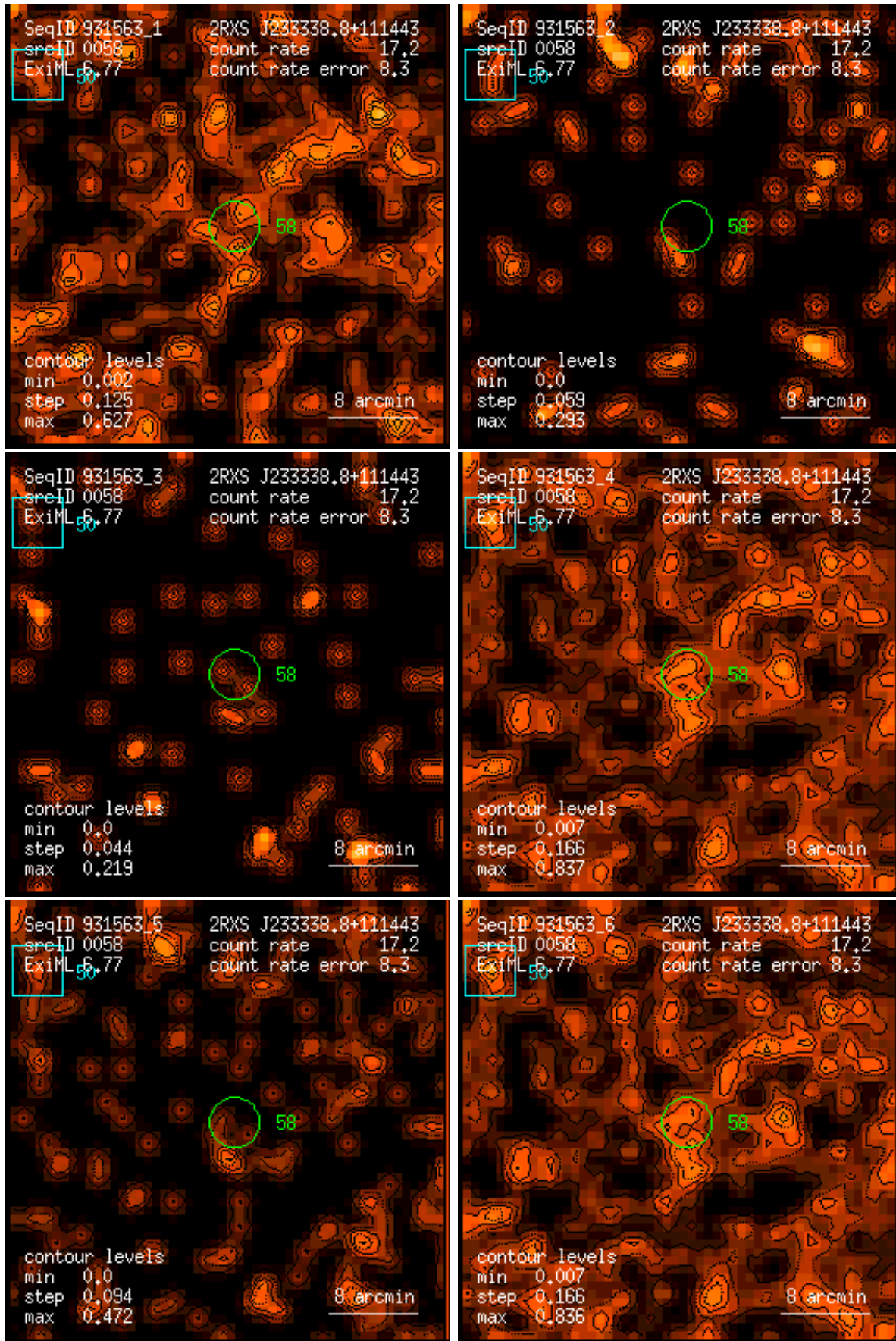
Figure 58: RASS 931563: detection 0058: band rate images, Gaussian filter: (1) PSPC channels 11 – 41, (2) 52 – 90, (3) 91 – 201, (4) 11 – 235, (5) 52 – 201, (6) 11 – 201. Broad band rates in counts/ks. Band rate contour levels in counts/ks/arcmin 2 .
