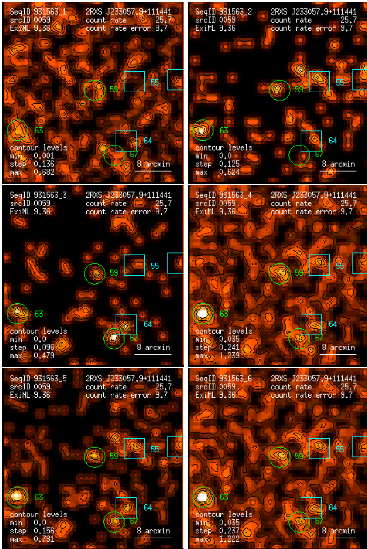
Figure 59: RASS 931563: detection 0059: band rate images, Gaussian filter: (1) PSPC channels 11 – 41, (2) 52 – 90, (3) 91 – 201, (4) 11 – 235, (5) 52 – 201, (6) 11 – 201. Broad band rates in counts/ks. Band rate contour levels in counts/ks/arcmin 2 .
