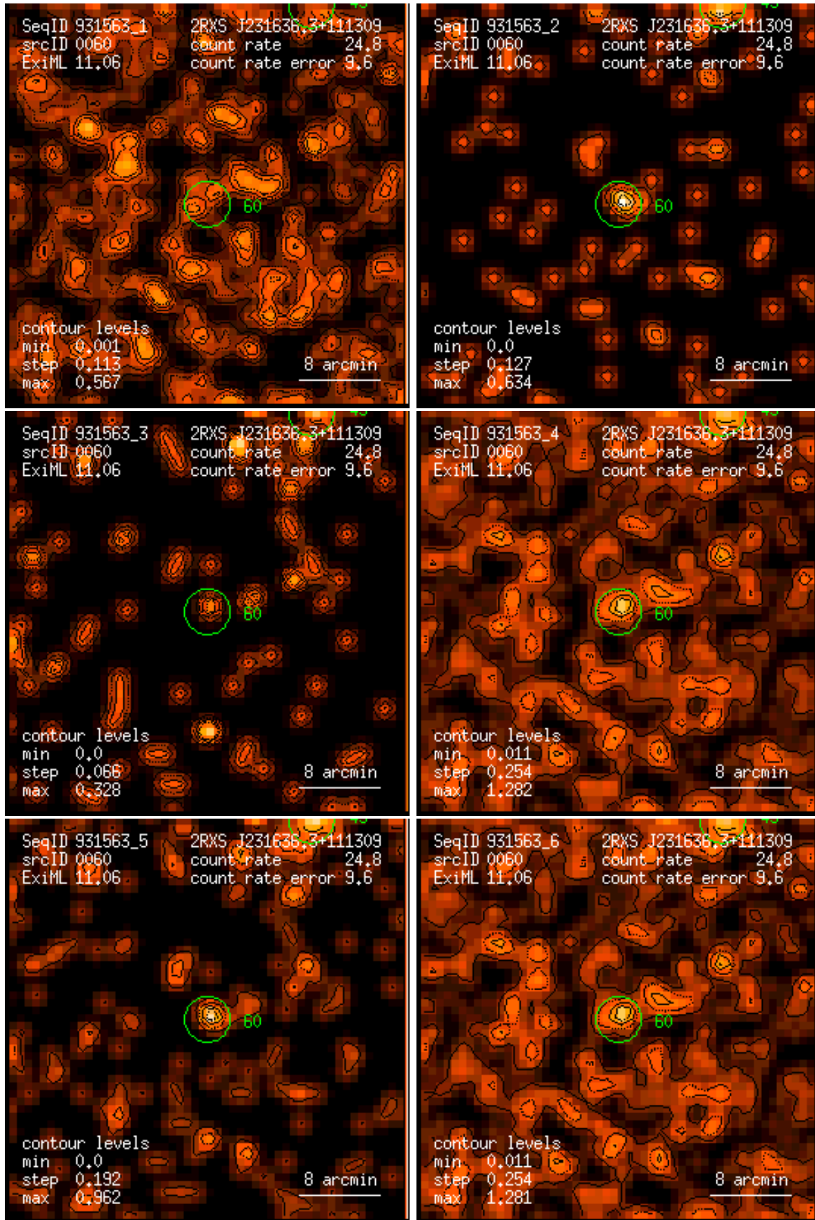
Figure 60: RASS 931563: detection 0060: band rate images, Gaussian filter: (1) PSPC channels 11 – 41, (2) 52 – 90, (3) 91 – 201, (4) 11 – 235, (5) 52 – 201, (6) 11 – 201. Broad band rates in counts/ks. Band rate contour levels in counts/ks/arcmin 2 .
