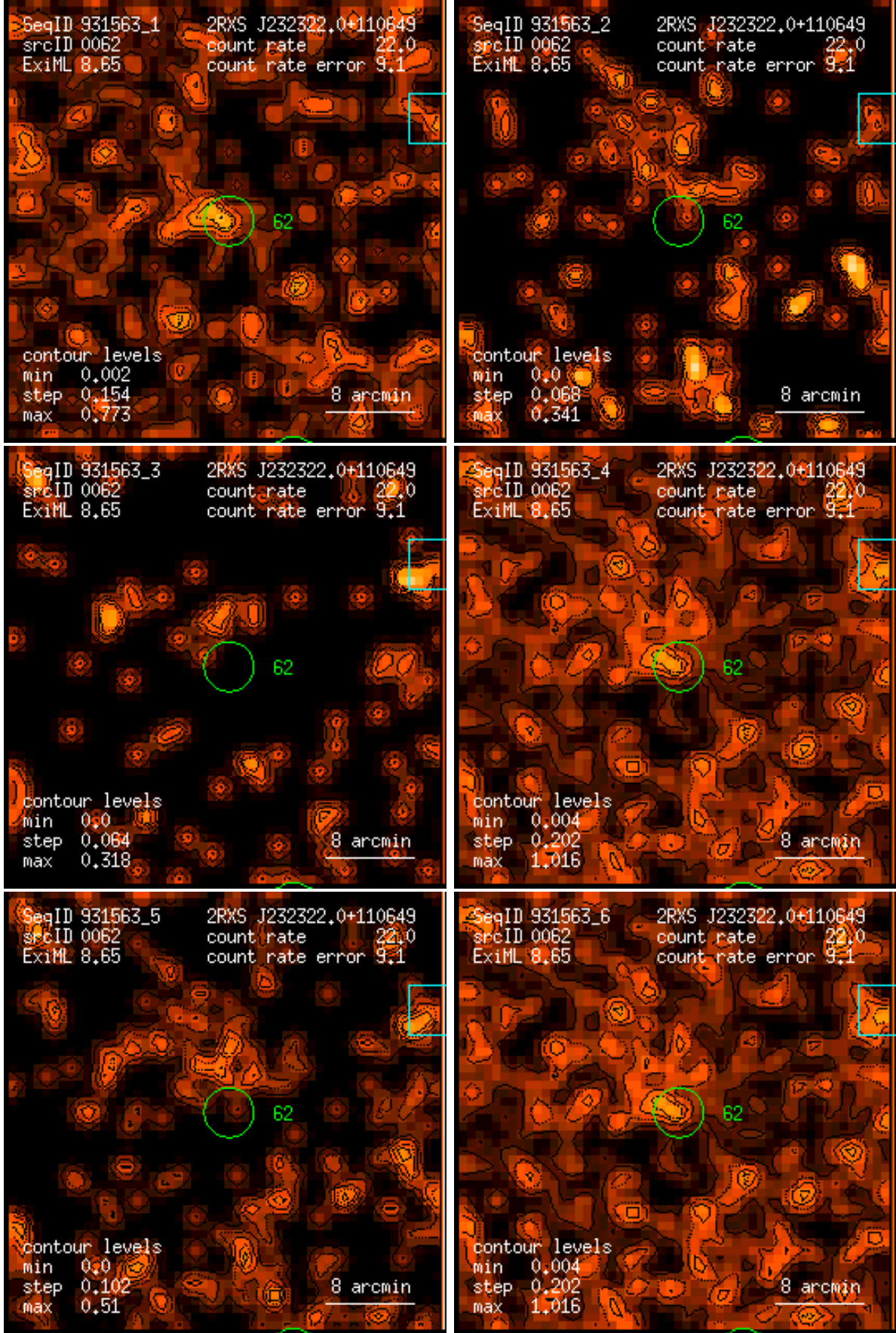
Figure 62: RASS 931563: detection 0062: band rate images, Gaussian filter: (1) PSPC channels 11 – 41, (2) 52 – 90, (3) 91 – 201, (4) 11 – 235, (5) 52 – 201, (6) 11 – 201. Broad band rates in counts/ks. Band rate contour levels in counts/ks/arcmin 2 .
