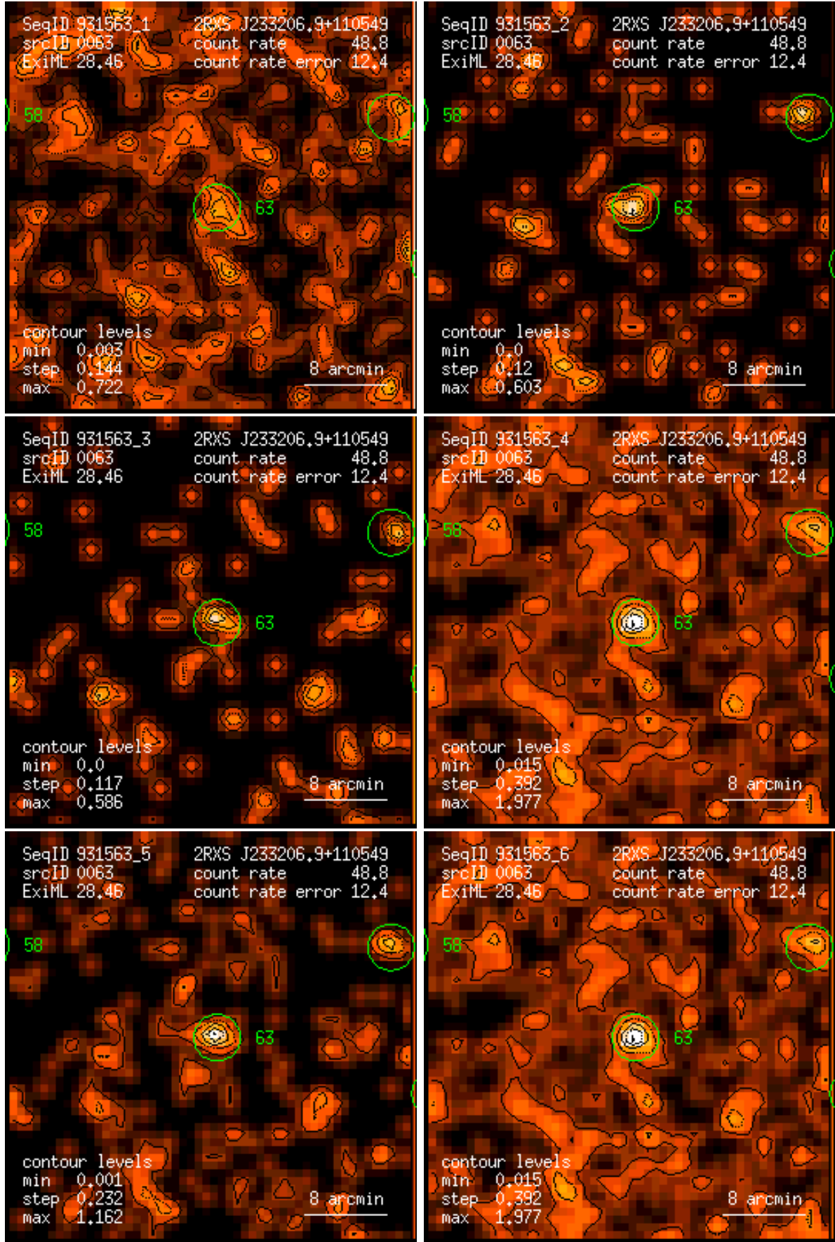
Figure 63: RASS 931563: detection 0063: band rate images, Gaussian filter: (1) PSPC channels 11 – 41, (2) 52 – 90, (3) 91 – 201, (4) 11 – 235, (5) 52 – 201, (6) 11 – 201. Broad band rates in counts/ks. Band rate contour levels in counts/ks/arcmin 2 .
