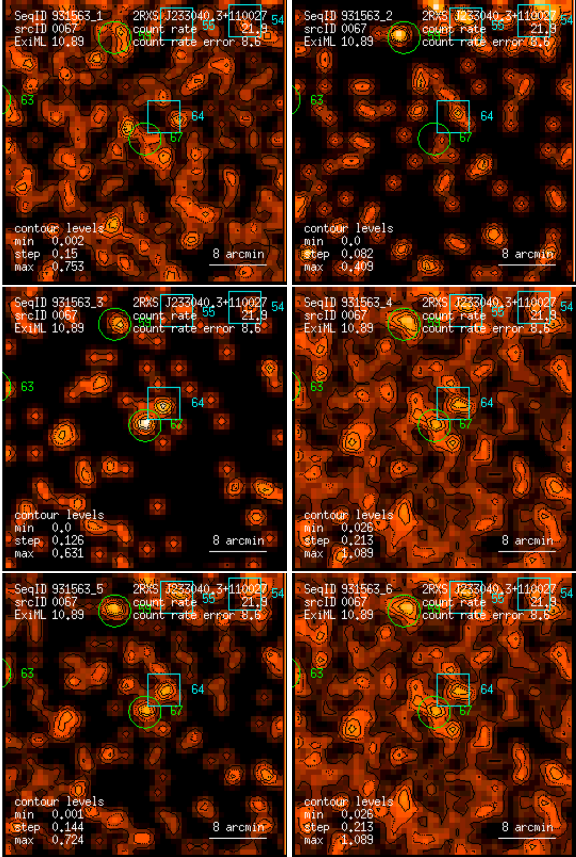
Figure 67: RASS 931563: detection 0067: band rate images, Gaussian filter: (1) PSPC channels 11 – 41, (2) 52 – 90, (3) 91 – 201, (4) 11 – 235, (5) 52 – 201, (6) 11 – 201. Broad band rates in counts/ks. Band rate contour levels in counts/ks/arcmin 2 .
